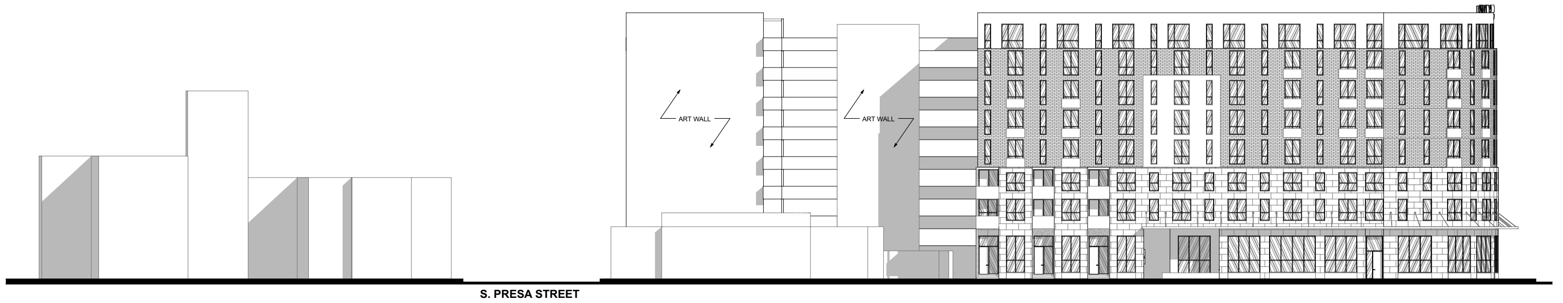
north elevation
