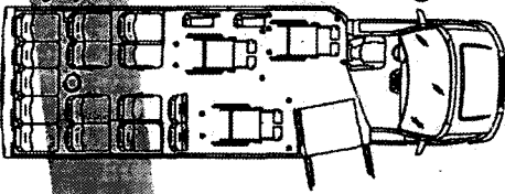
26ft, 191" WB - 18 Passenger
