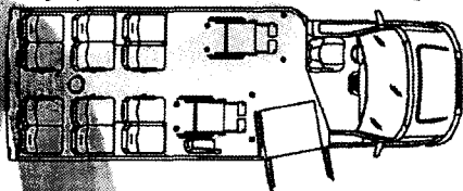
26ft, 191" WB - 19 Passenger
