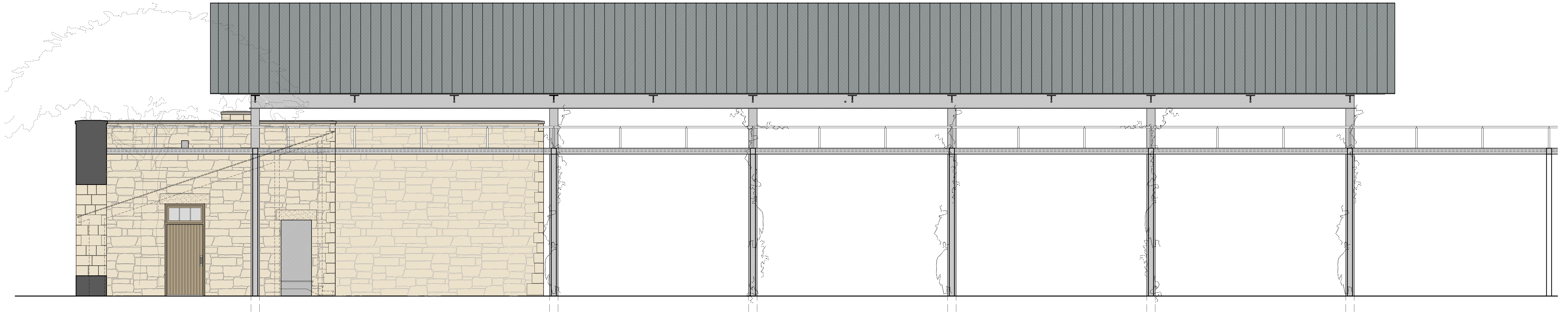
1 North Parking Lot Elevation - West (w/Pergola) Scale: 1/4"=1'-0"
