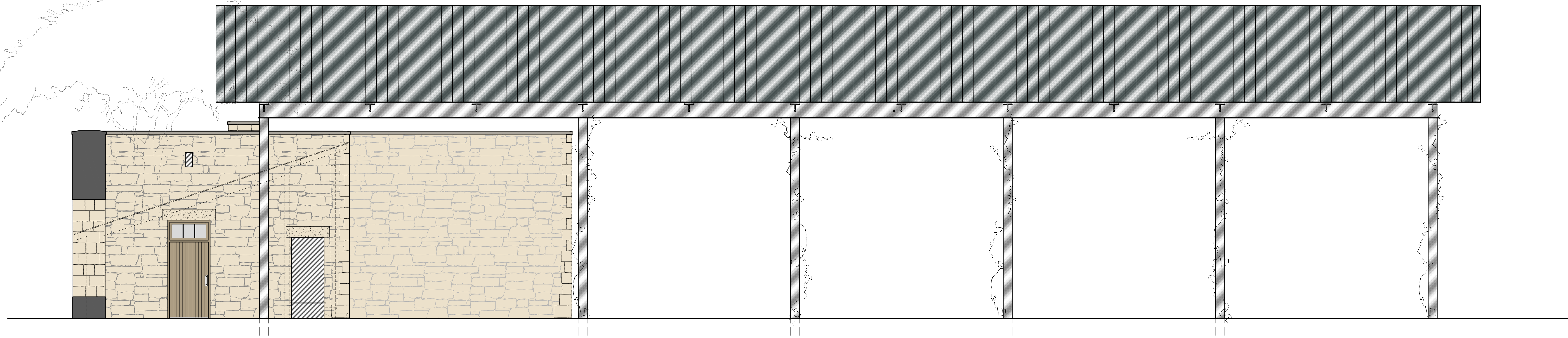
3 Wall Shed & Storage - West @ Parking Lot Scale: 1/4"=1'-0"
