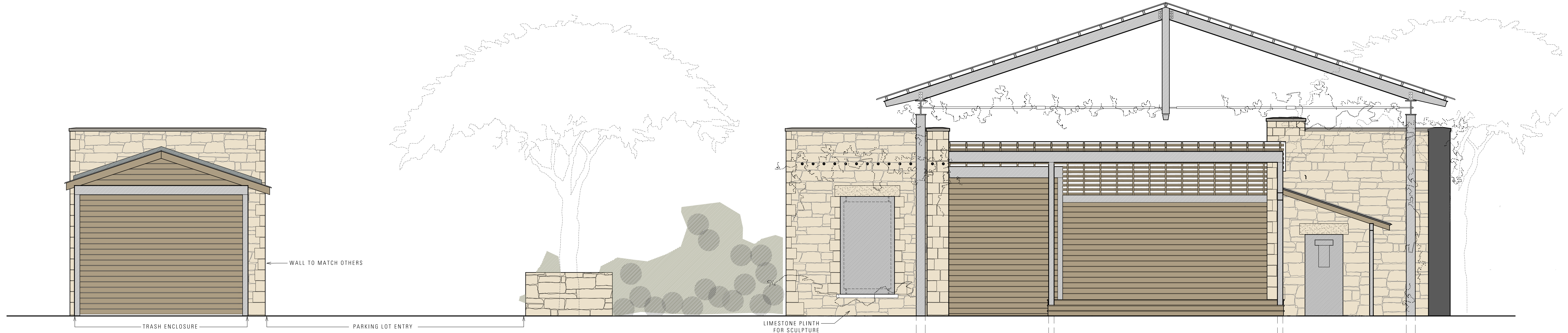
2 North Parking Lot Elevation - South (Parking Lot Interior) Scale: 1/4"=1'-0"
