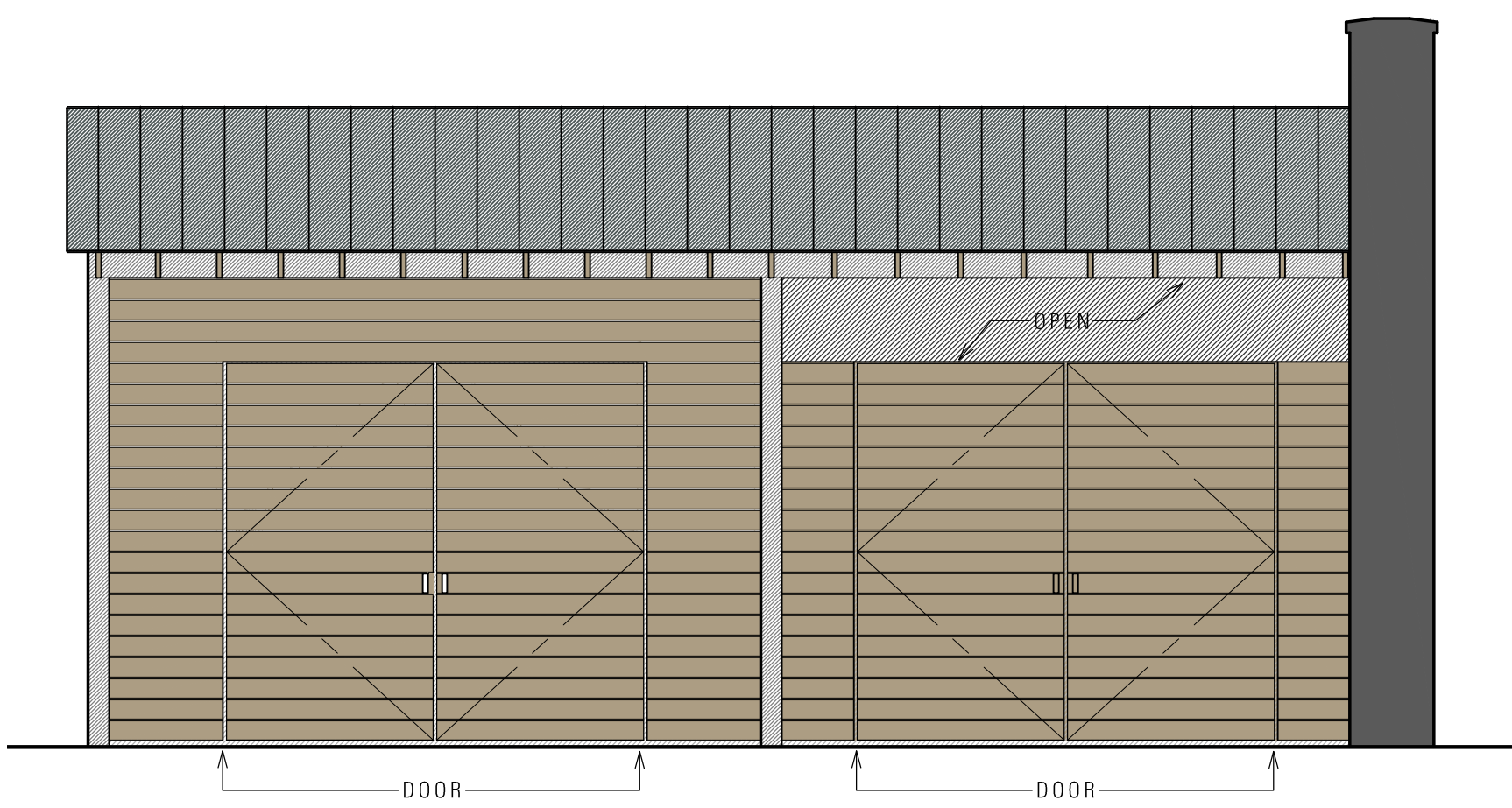
3 Trash Enclosure - East Elevation Scale: 1/4"=1'-0"
