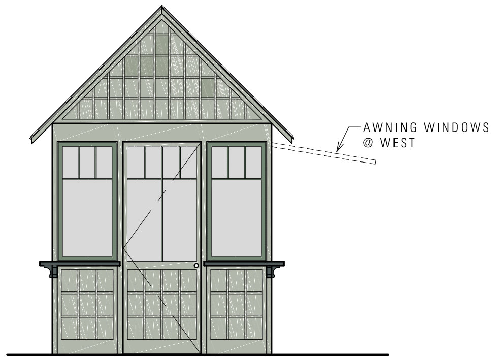
5 Courtyard Bar - North & South Scale: 1/4"=1'-0"
