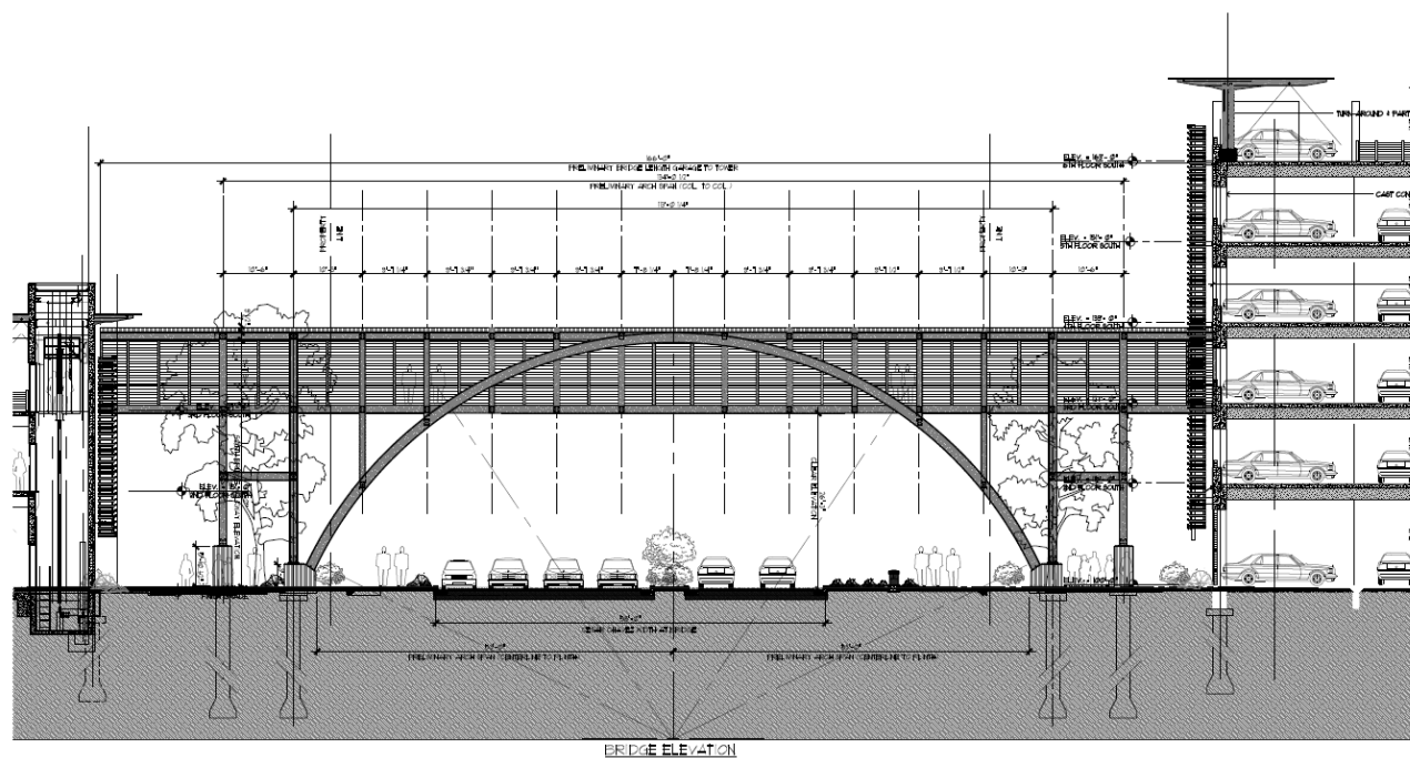
1 PRELIMINARY BRIDGE ELEVATION SCALE: GRAPHIC SCALE
