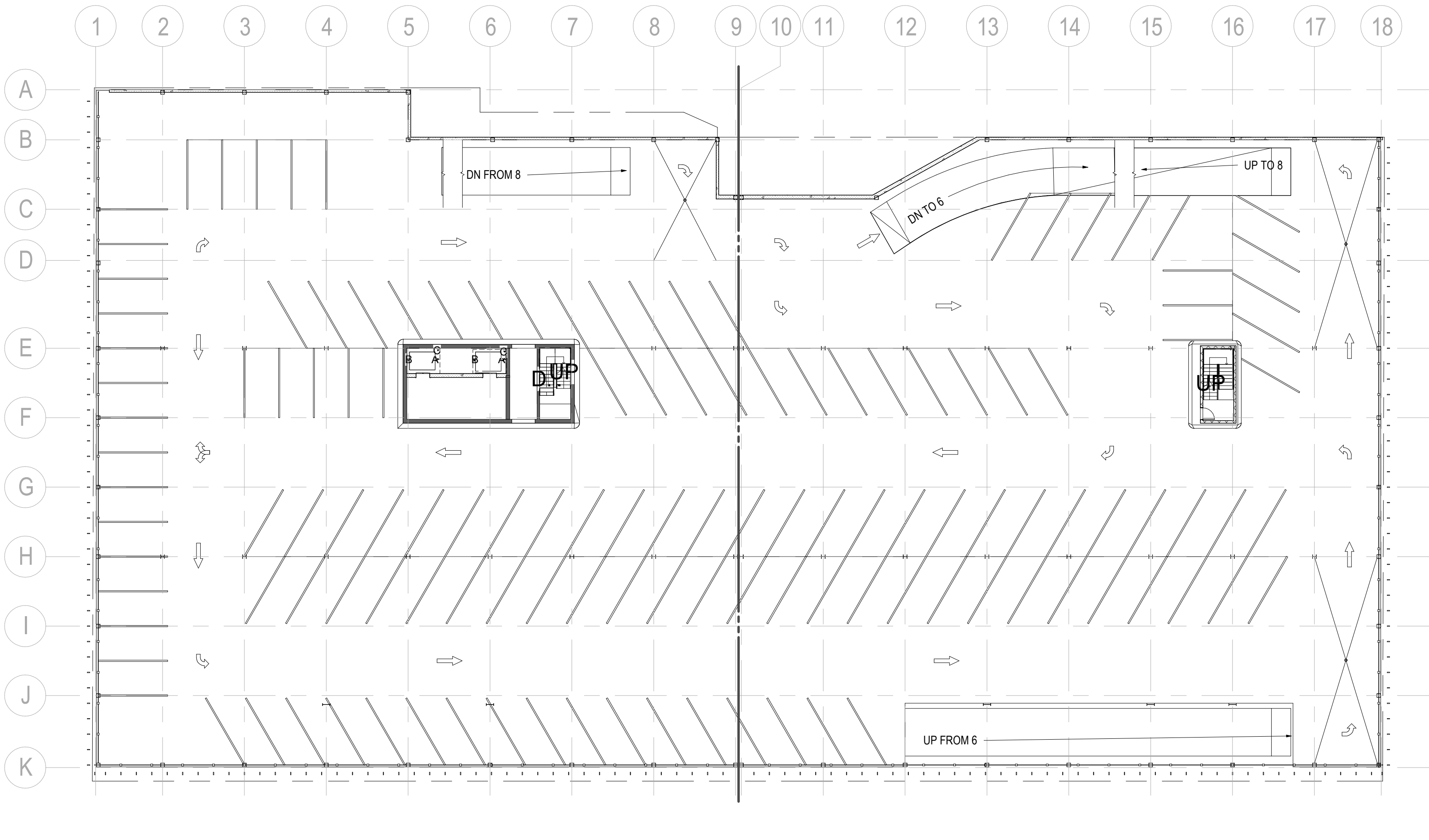
3 LEVEL 07 (NEW) SCALE: 3/64" = 1'-0"
