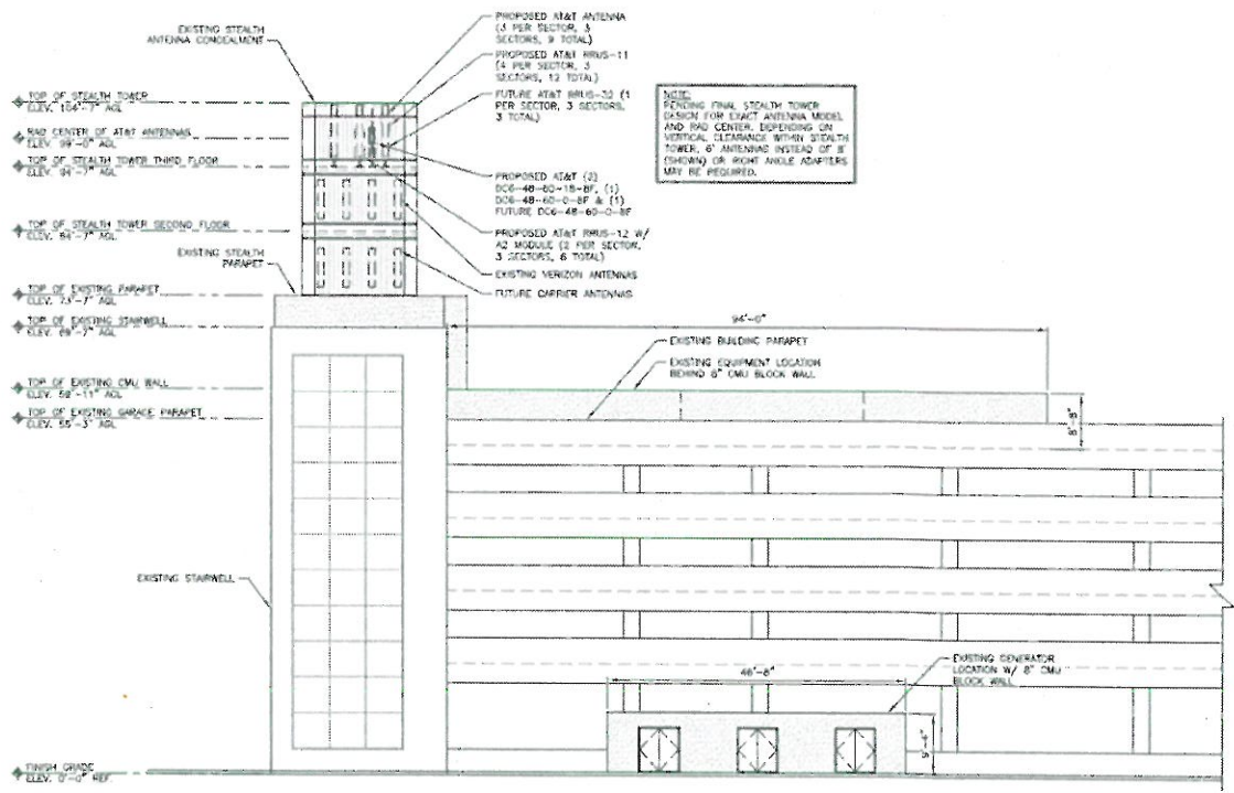
1 PROPOSED ELEVATION FULL SIZE PLOT SCALE: 1/8" = 1'-0" HALF SIZE PLOT SCALE: 1/16" = 1'-0" 0 4 8 16'
