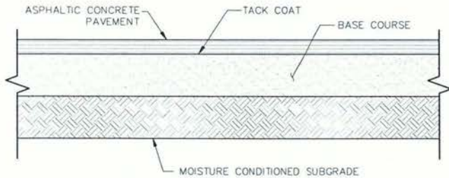
UNIVERSITY PASS - FLEXIBLE PAVEMENT SECTIONS NOT TO SCALE
