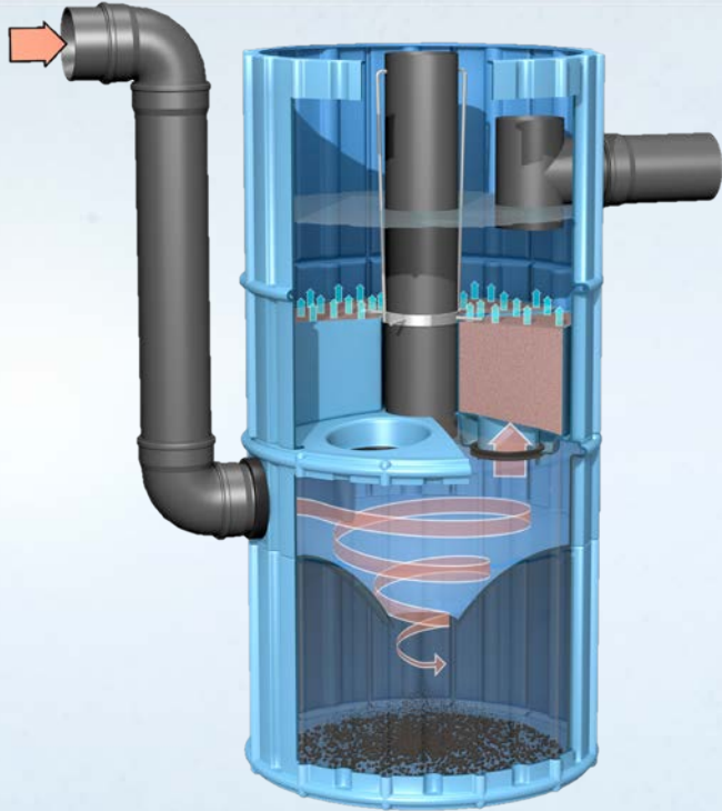
Trash Filtration
