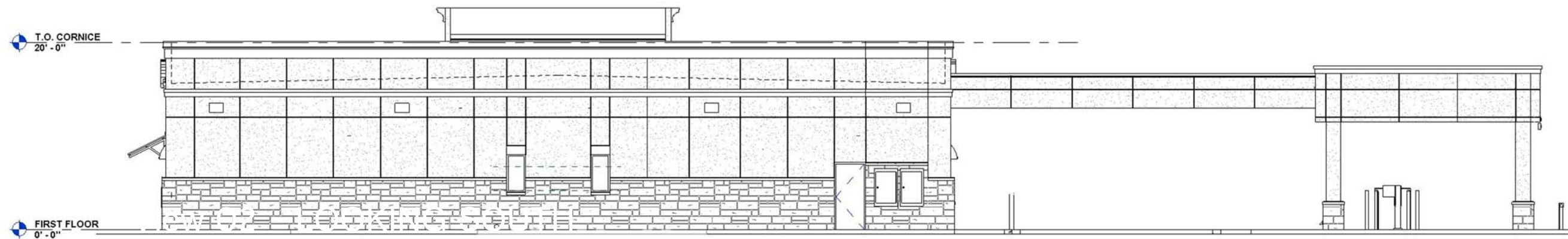
SOUTH VIEW
