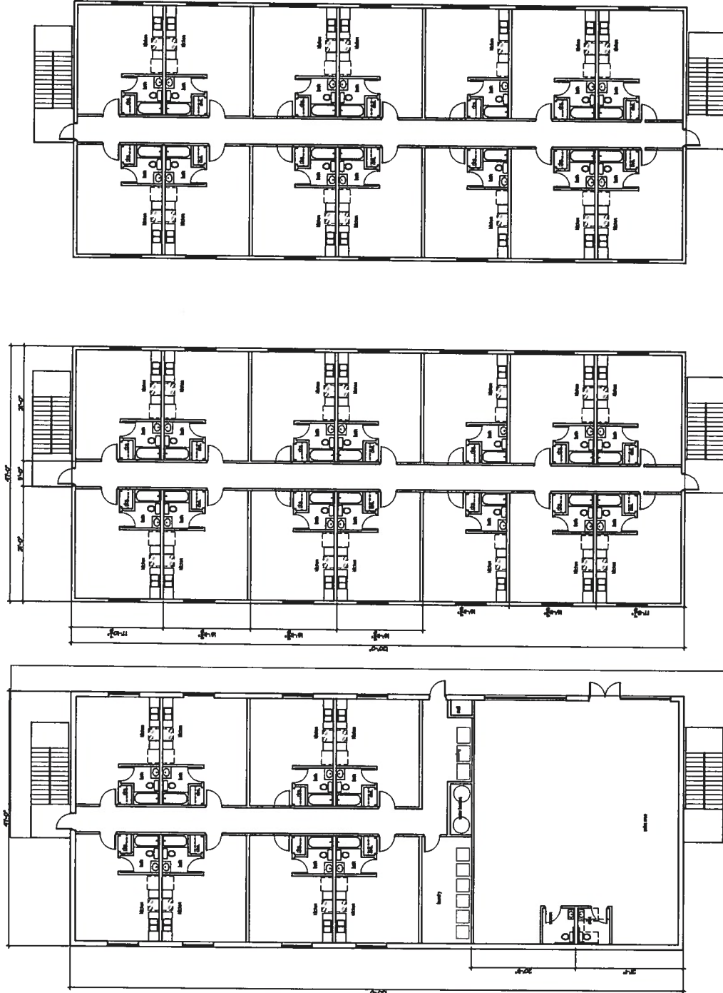
03 third floor plan
