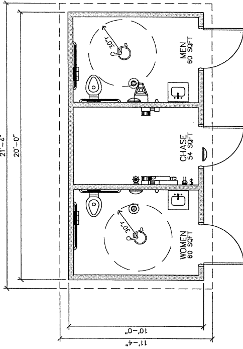
FLOOR PLAN
