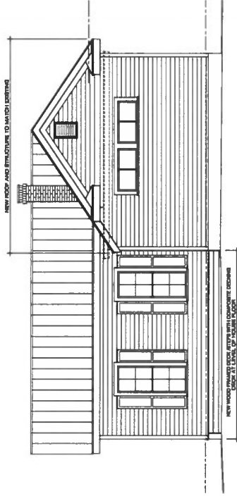
2 New Construction North Elevation 1/4" = 1'-0"
