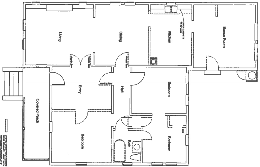
1 Existing Floor Plan 1/4" = 1'-0"
