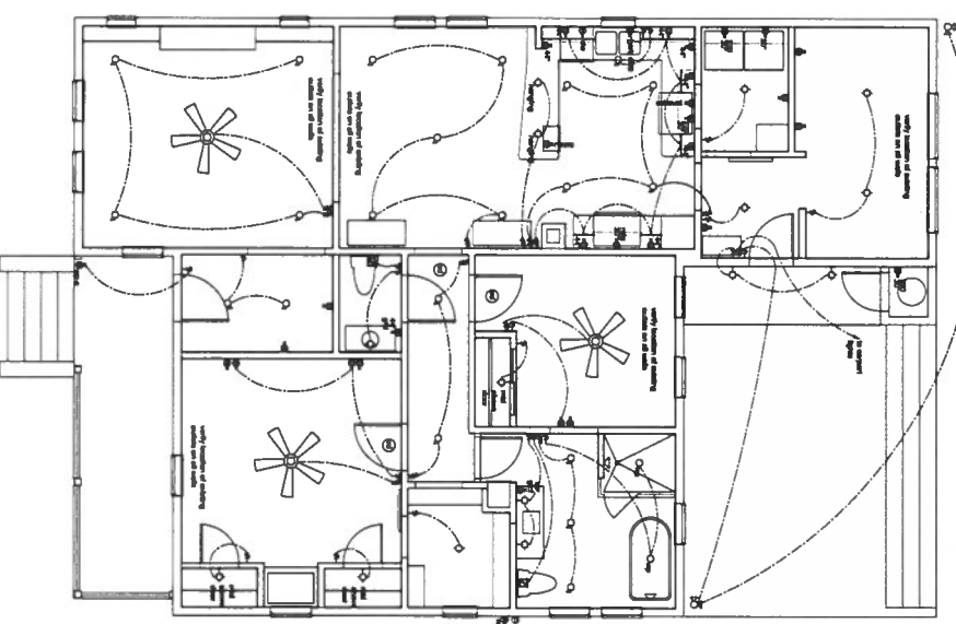
3 Electrical Floor Plan 1/4" = 1'-0"
