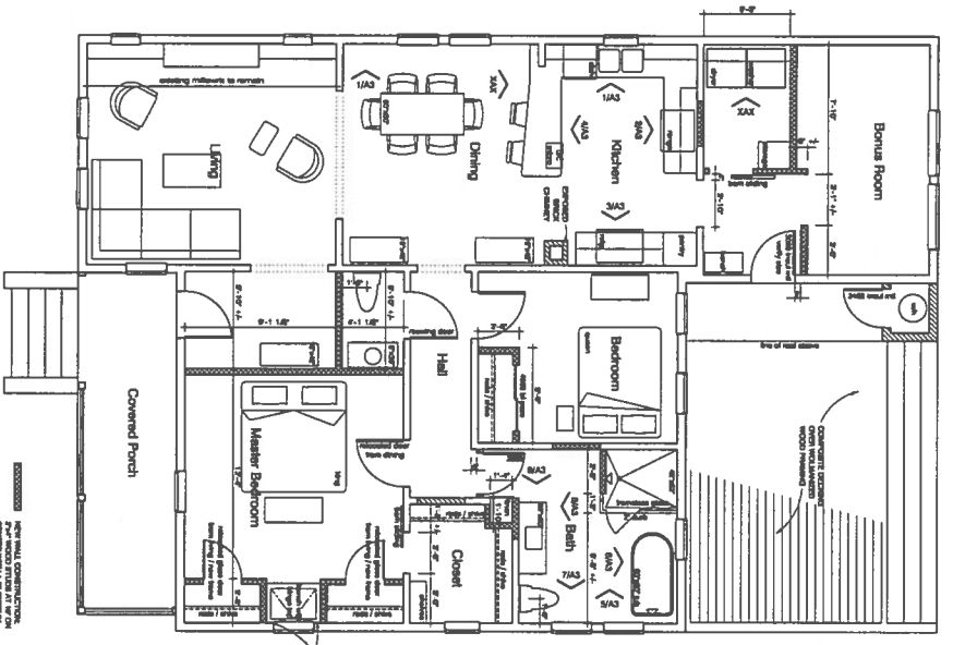
2 New Construction Floor Plan 1/4" = 1'-0"
