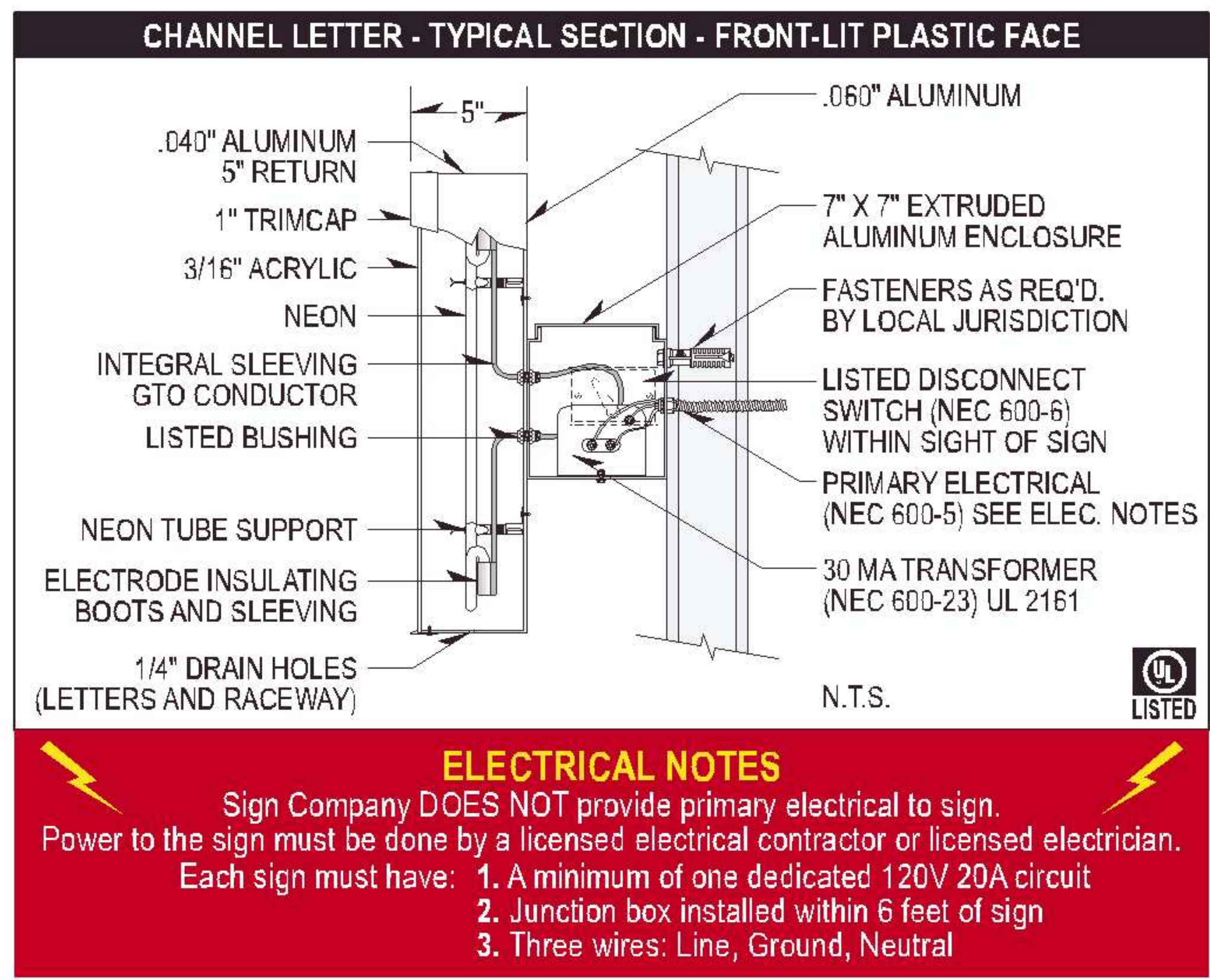
SECTION VIEW
