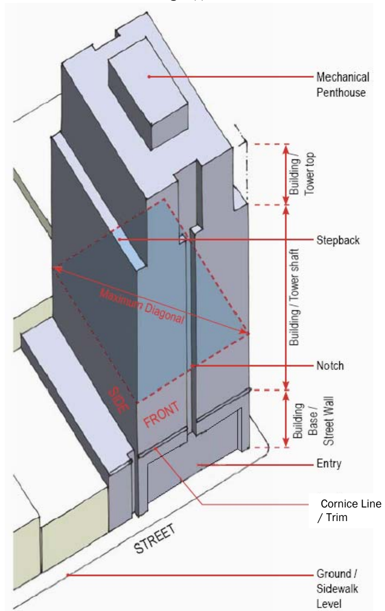
Fig 5.8 Tower Massing & Bulk Control
