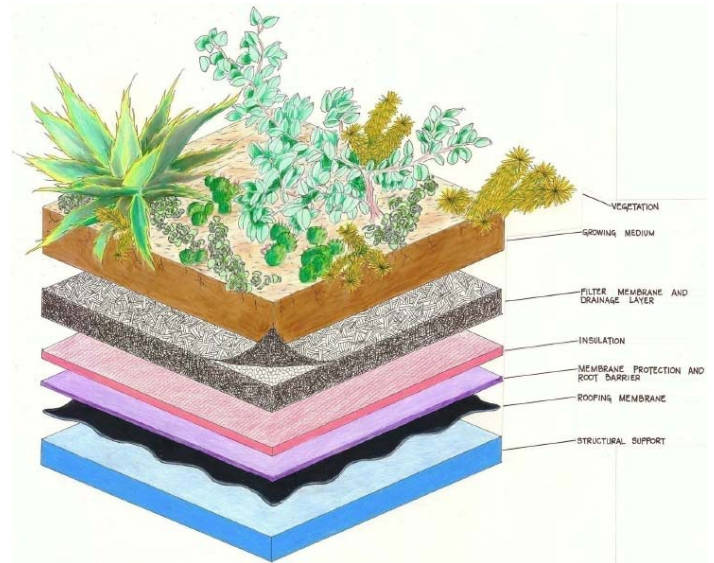
Fig 11.6 Roof Layers for a Green Roof Garden
