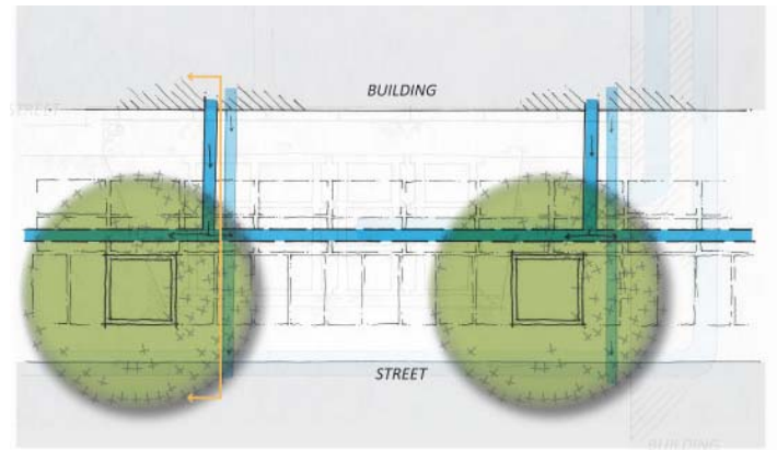
Fig 11.3 Rainleader Illustration Plan
