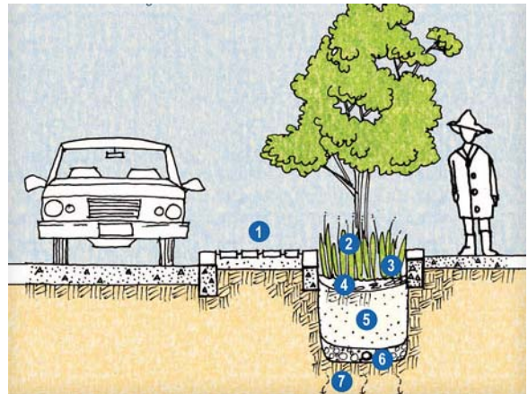
Fig 11.10 Curbside Flow-Through Planter 1 Pavers 2 Vegetation 3 New Tree 4 Mulch Layer 5 Newly Prepared Soil 6 Root Drainage 7 Undisturbed Native Soil
