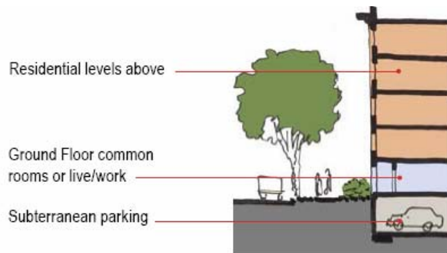
Fig 4.3 Residential Street Subterranean Parking
