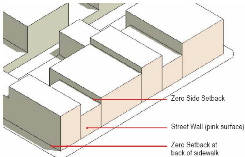
Fig 5.5 Desirable Street Wall and Setbacks
