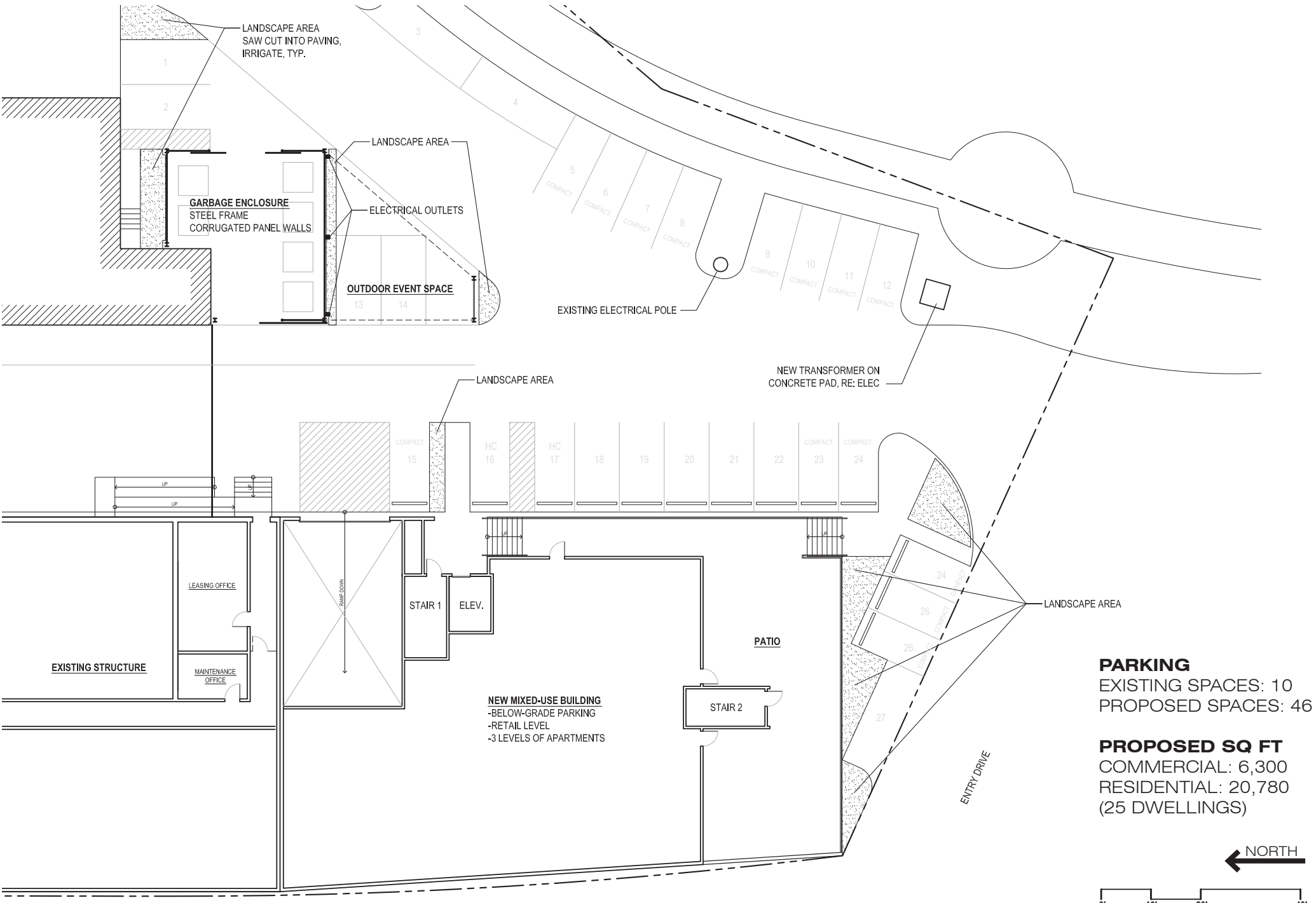
SITE PLAN
