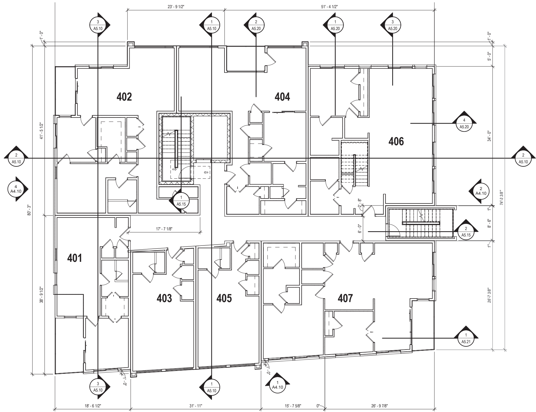
FOURTH FLOOR PLAN
