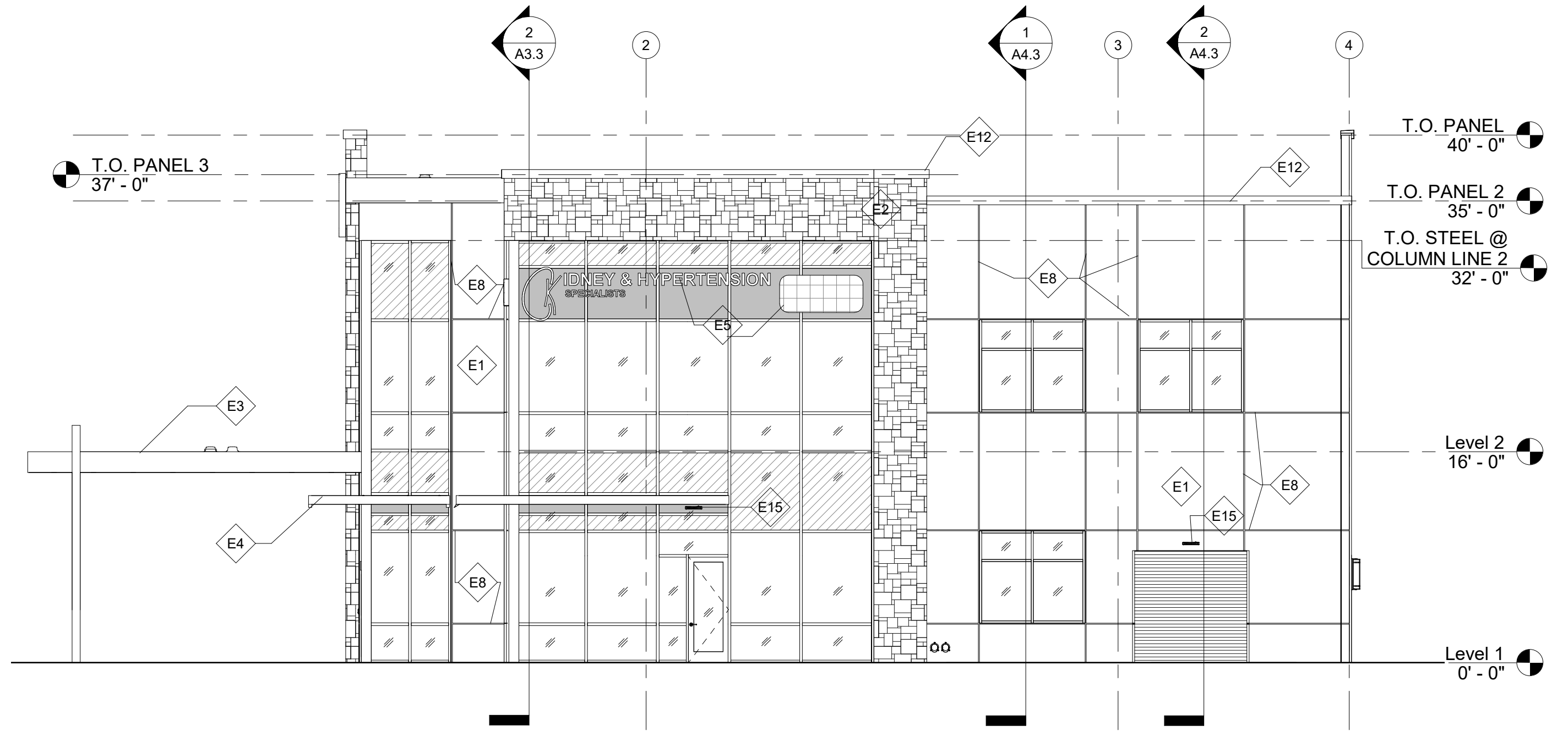
1 WEST EXTERIOR ELEVATION 1/8" = 1'-0"
