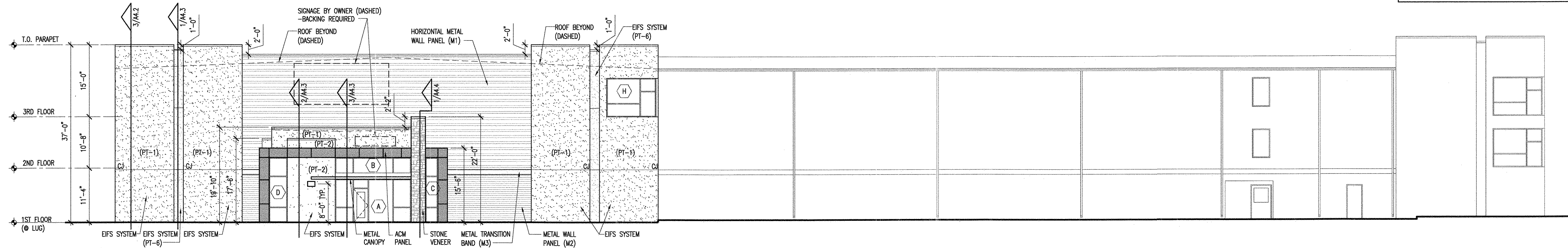
2 EAST ELEVATION SCALE: 3/32" = 1'-0"
