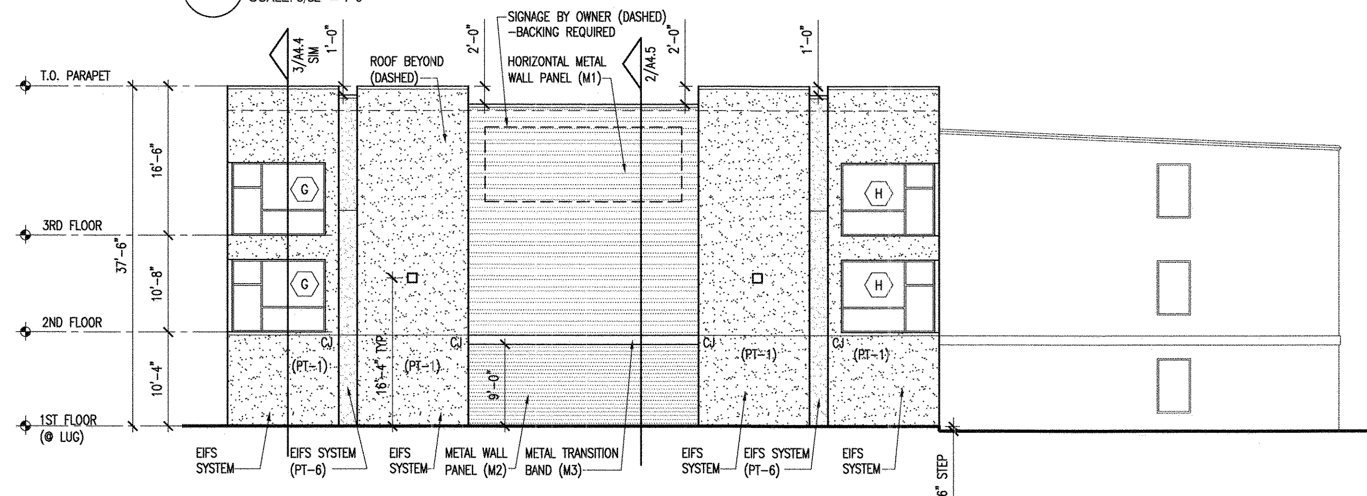
2 NORTH ELEVATION SCALE: 3/32" = 1'-0"
