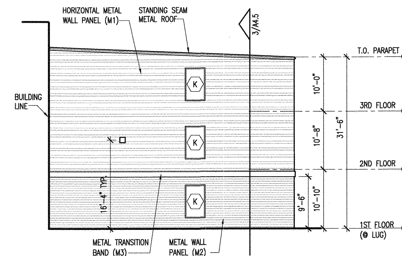
2A NORTH ELEVATION SCALE: 3/32" = 1'-0"
