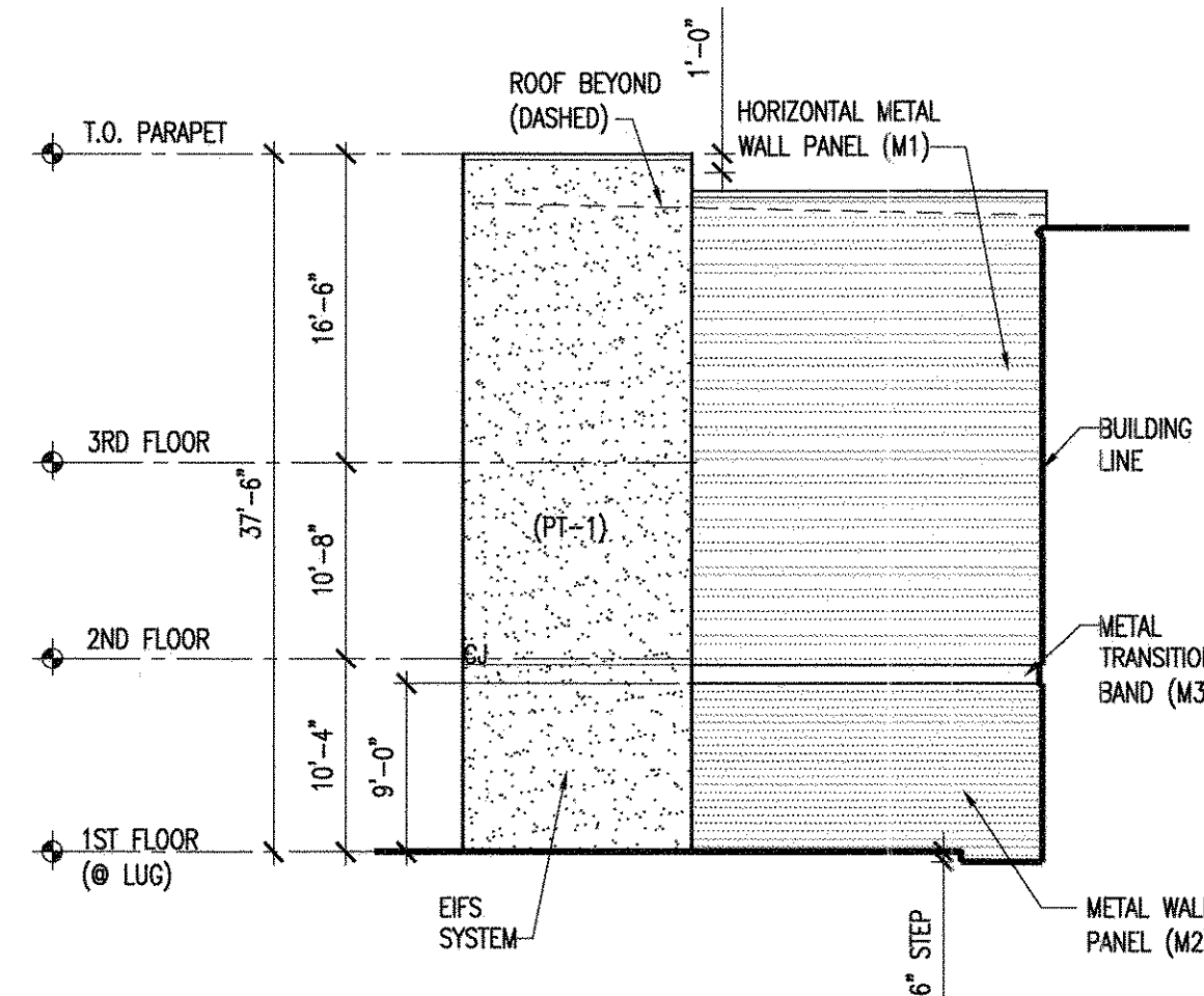
3A WEST ELEVATION SCALE: 3/32" = 1'-0"
