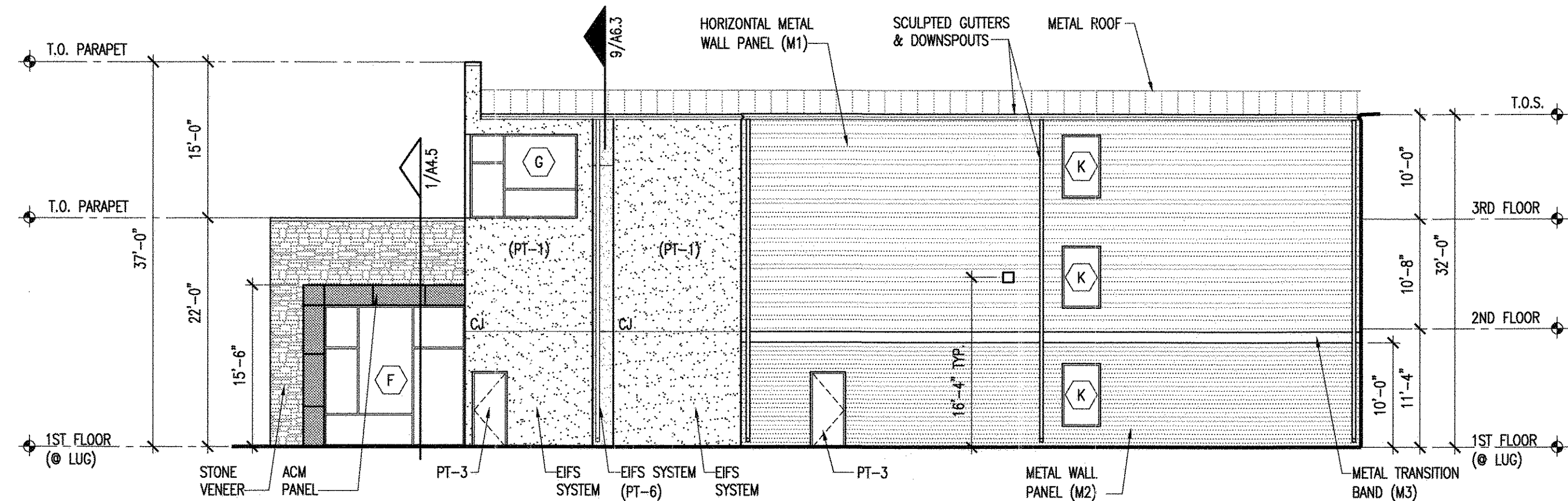
1 NORTH ELEVATION SCALE: 3/32" = 1'-0"
