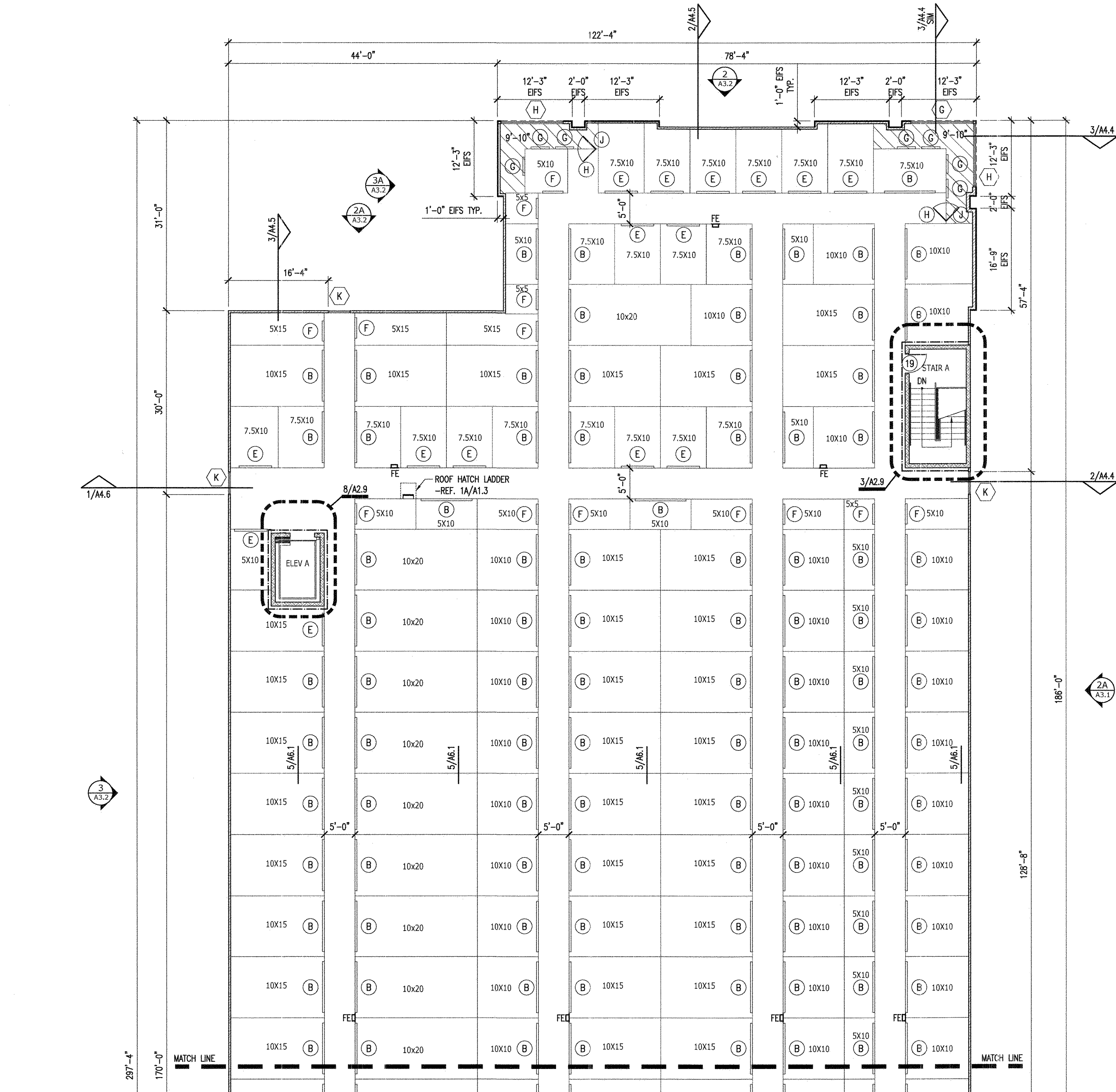
1 THIRD FLOOR PLAN SCALE: 3/32" = 1'-0"
