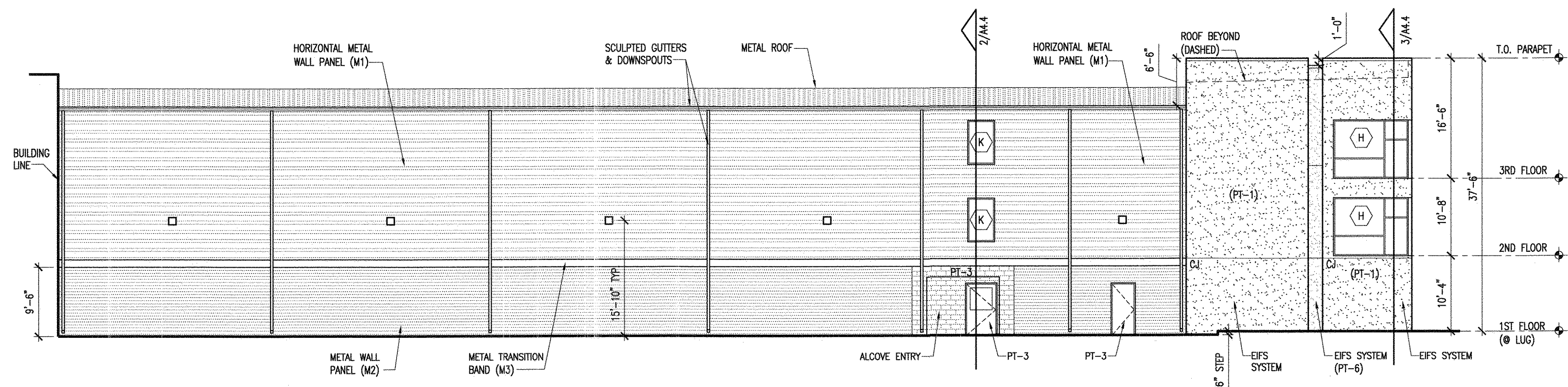
2A EAST ELEVATION SCALE: 3/32" = 1'-0"
