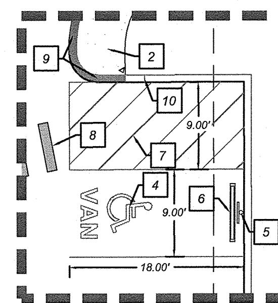
HANDICAP PARKING DETAIL "A"
