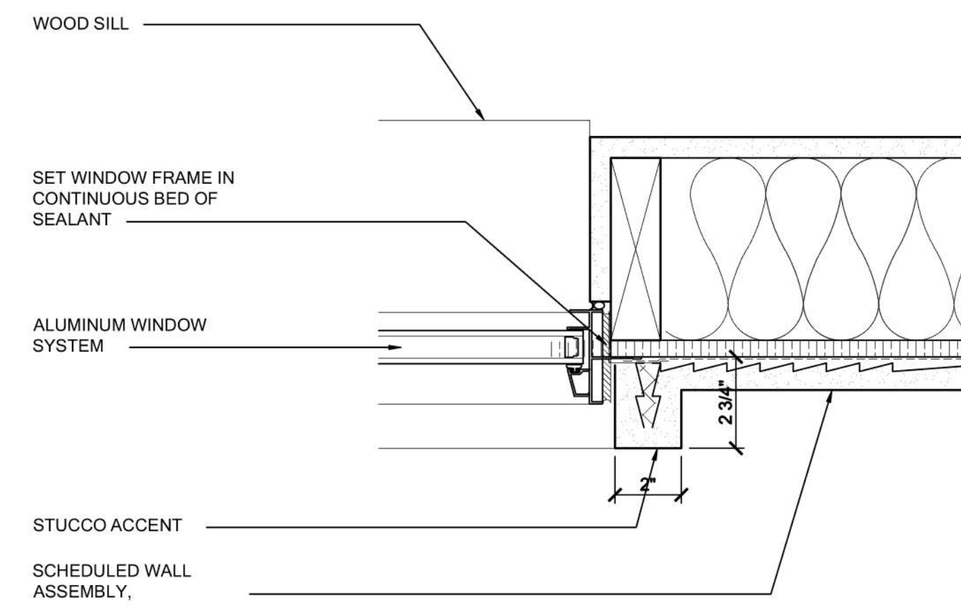
02 JAMB DETAIL AT CEMENT PLASTER
