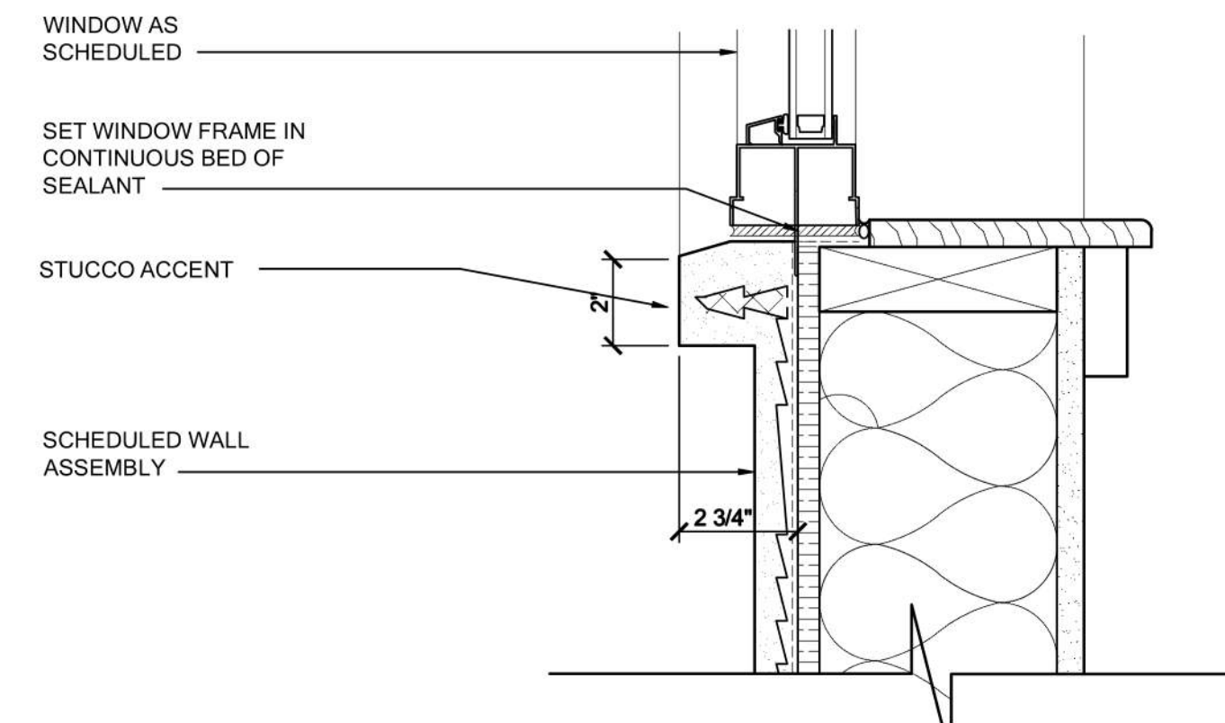
03 WINDOW SILL AT CEMENT PLASTER
