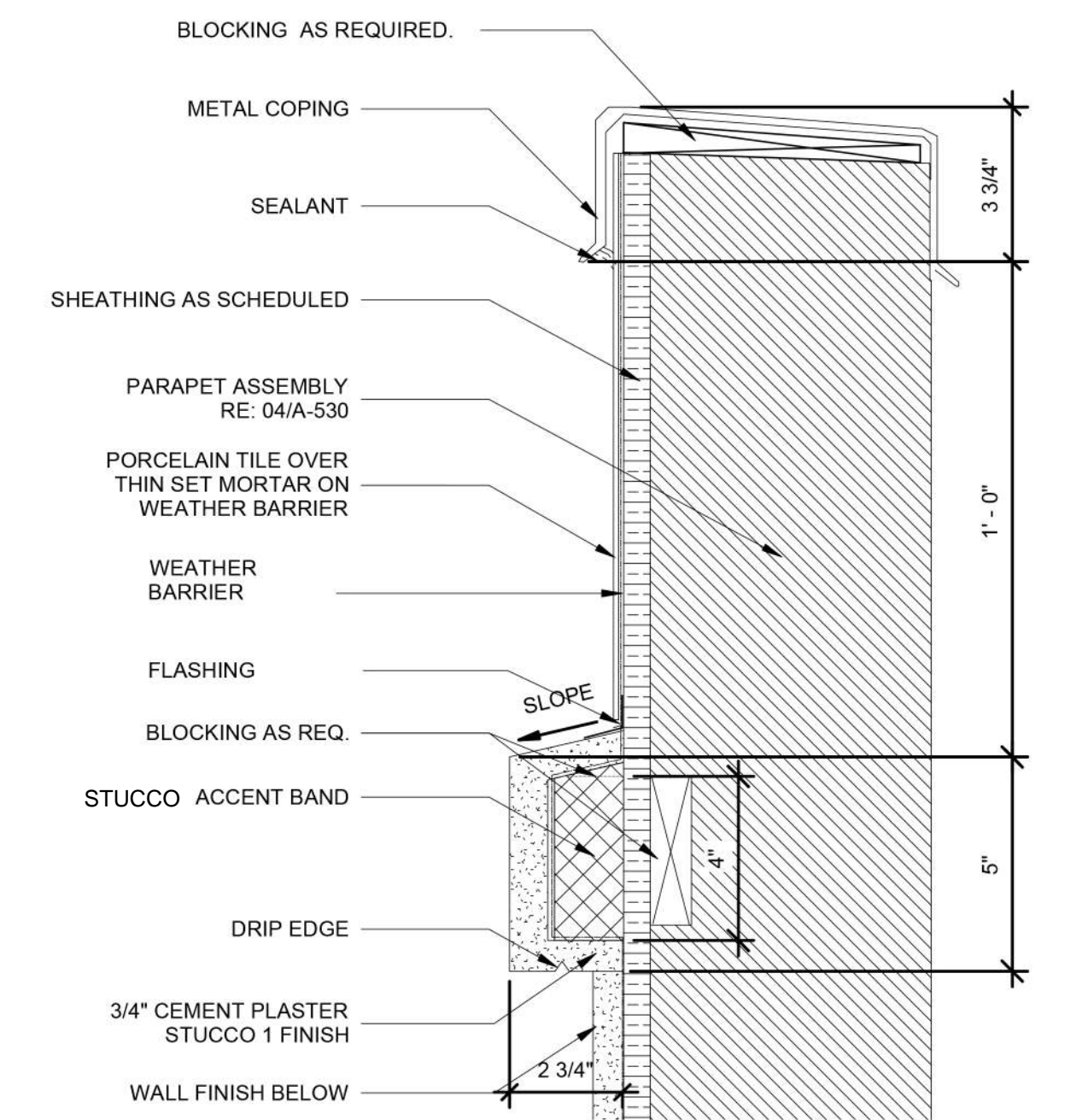
01 SECTION DETAIL
