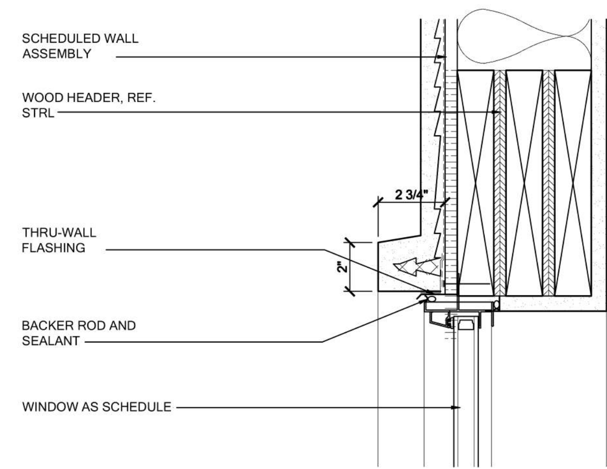
04 WINDOW HEAD AT CEMENT PLASTER
