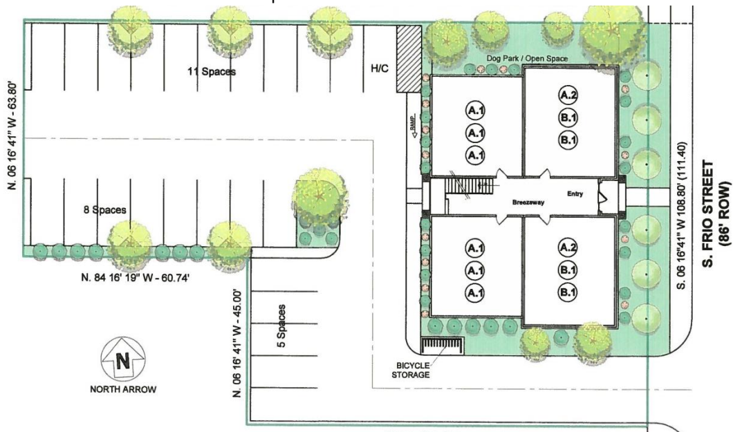
Preliminary Project Site Plan | 12 units
