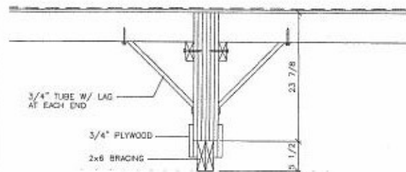
RIDGE BEAM BRACING DETAIL
