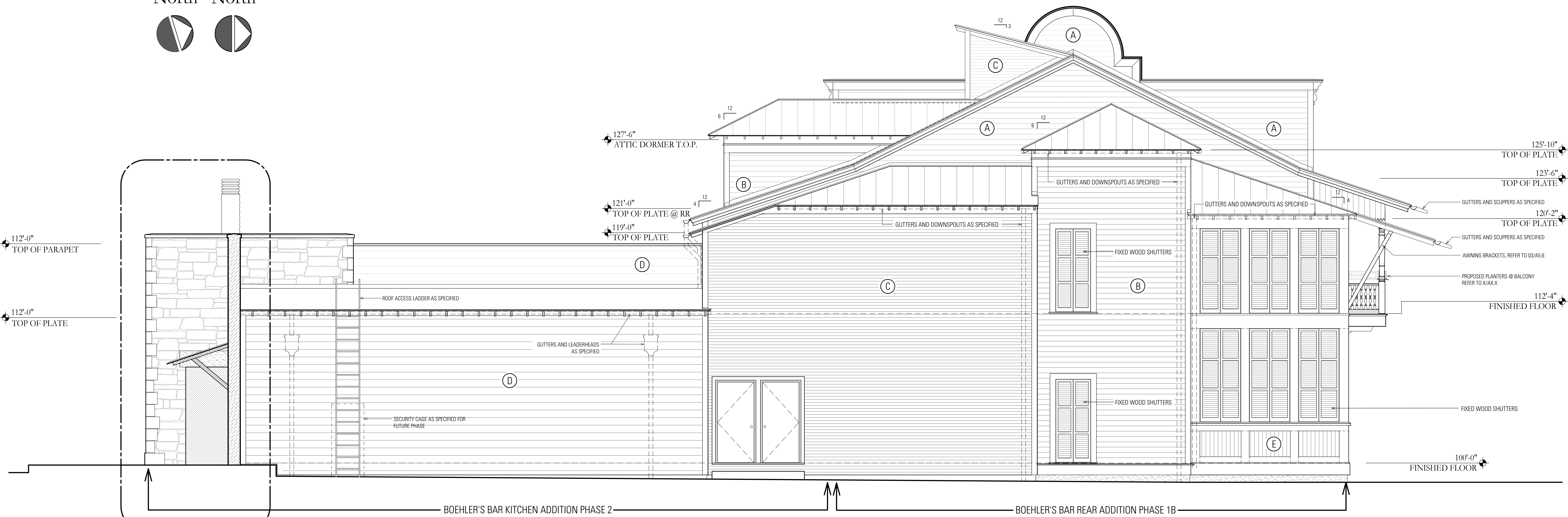
3 Boehler's Elevation - West Scale: 1/4"=1'-0"
