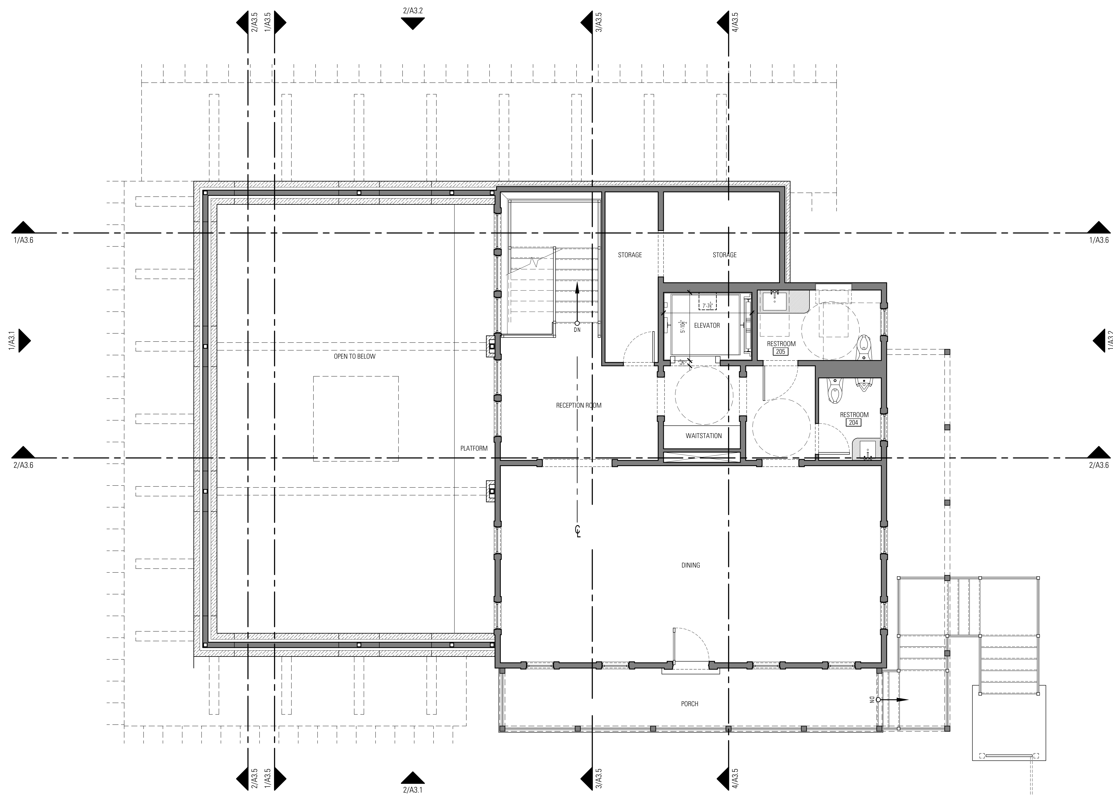
1 Floor Plan - Boehler's House Second Floor Scale: 1/4"=1'-0"
