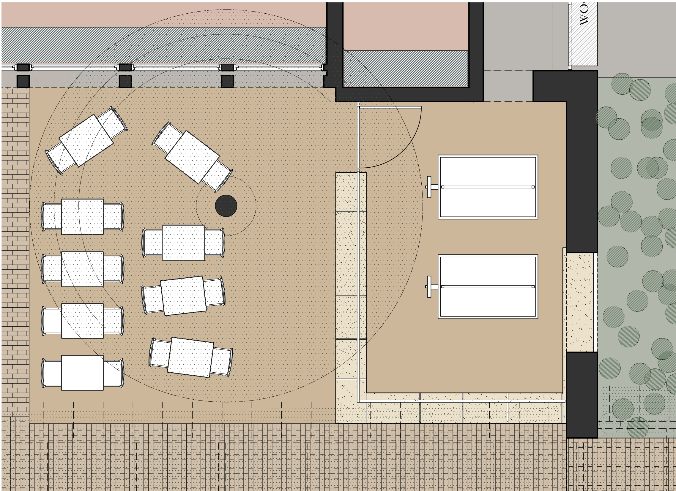
1 Boehler's Kitchen Service Plan Scale: 1/4"=1'-0"
