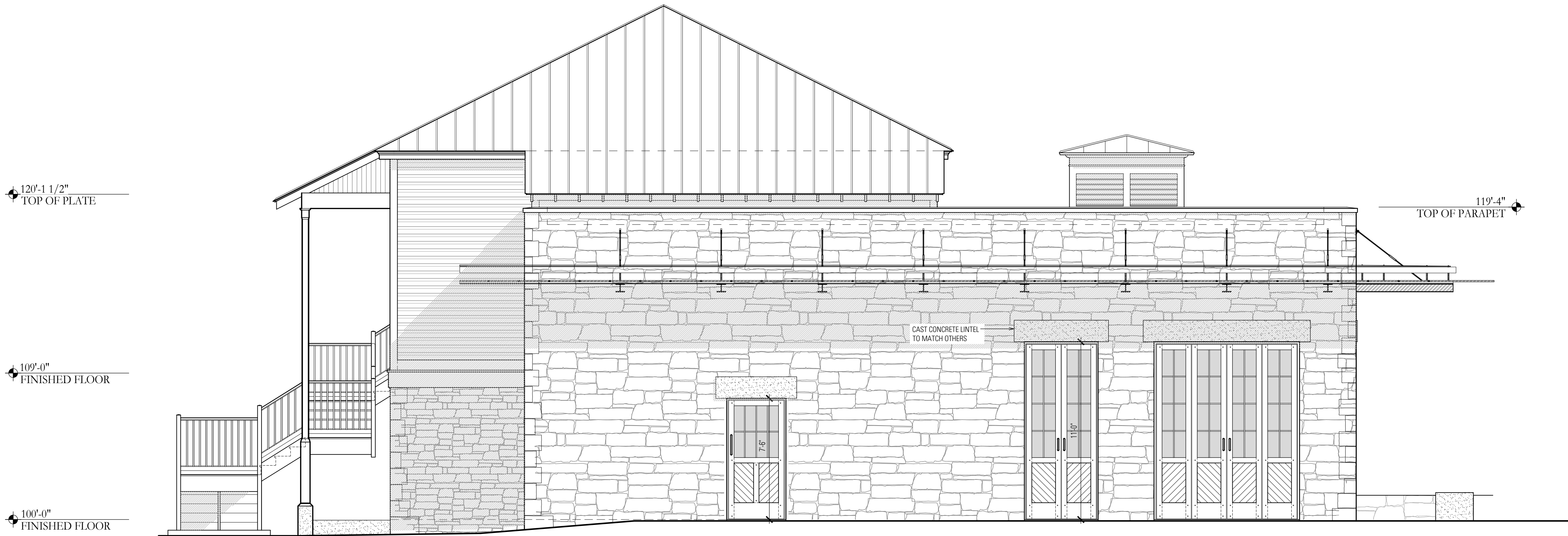
2 Elevation - West Scale: 1/4"=1'-0"
