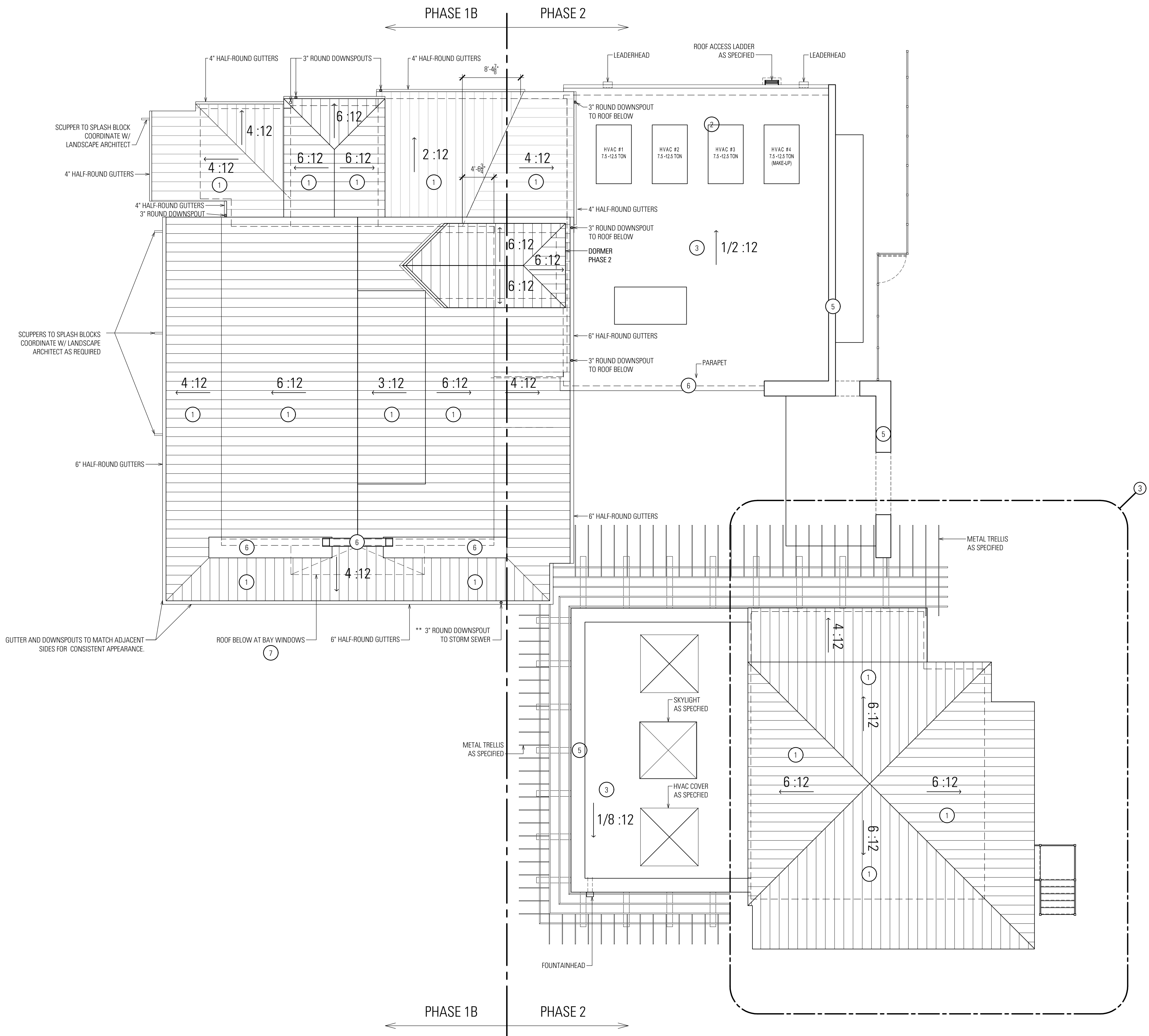
1 Boehler's Bar Roof Plan
