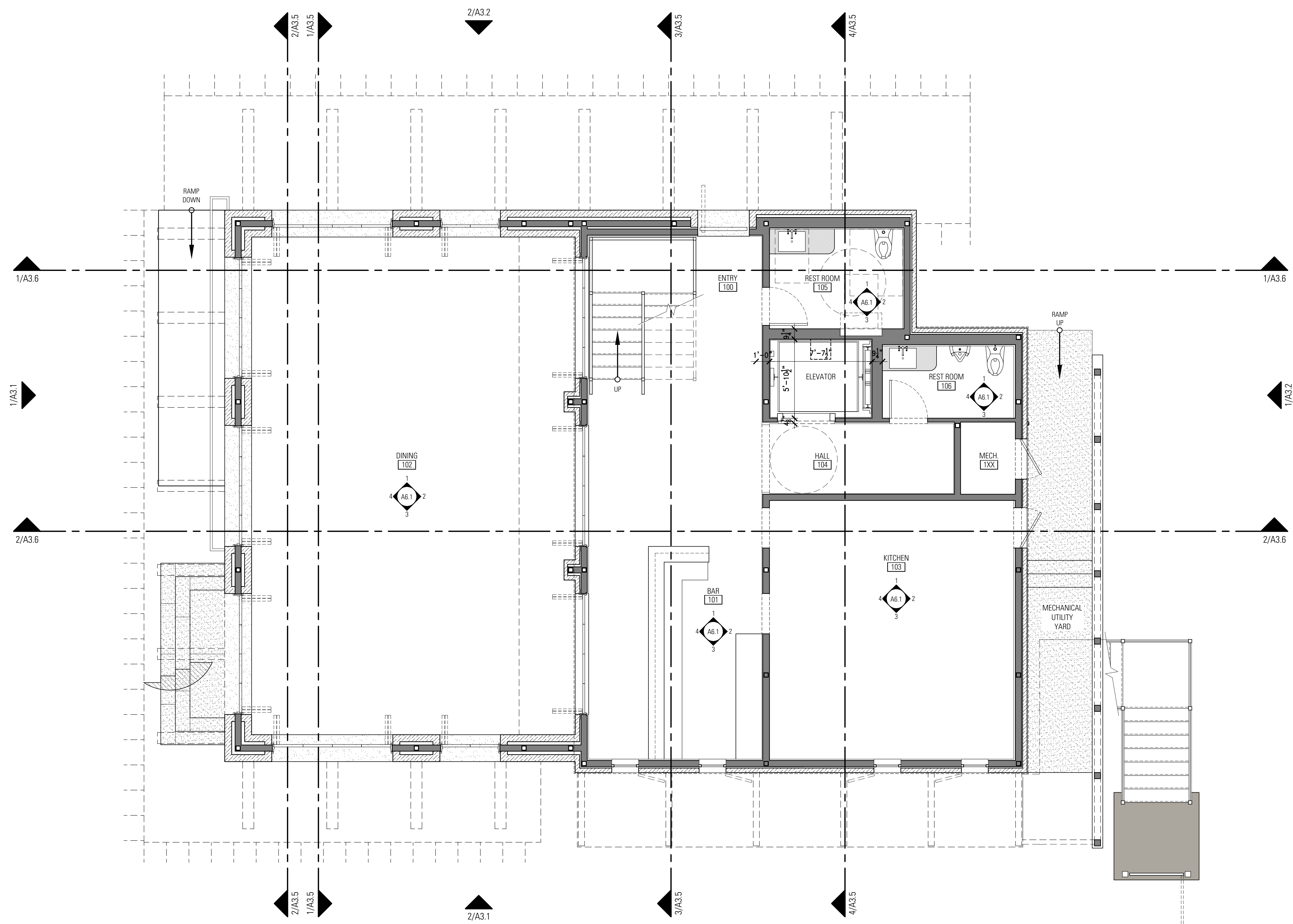
1 Floor Plan - Pavilion and Bar Scale: 1/4"=1'-0"
