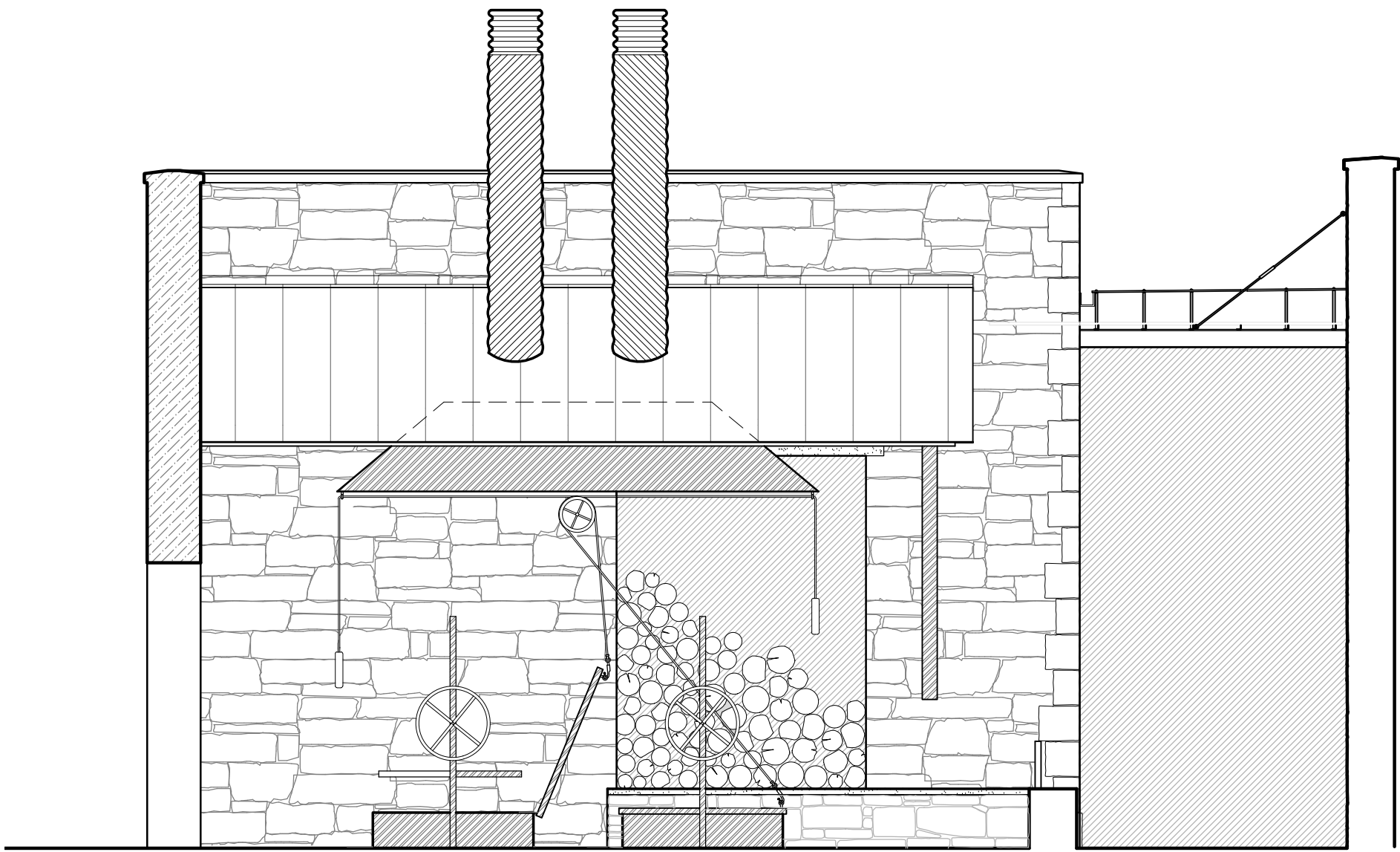
3 BBQ Pit North Elevation Scale: 1/4"=1'-0"
