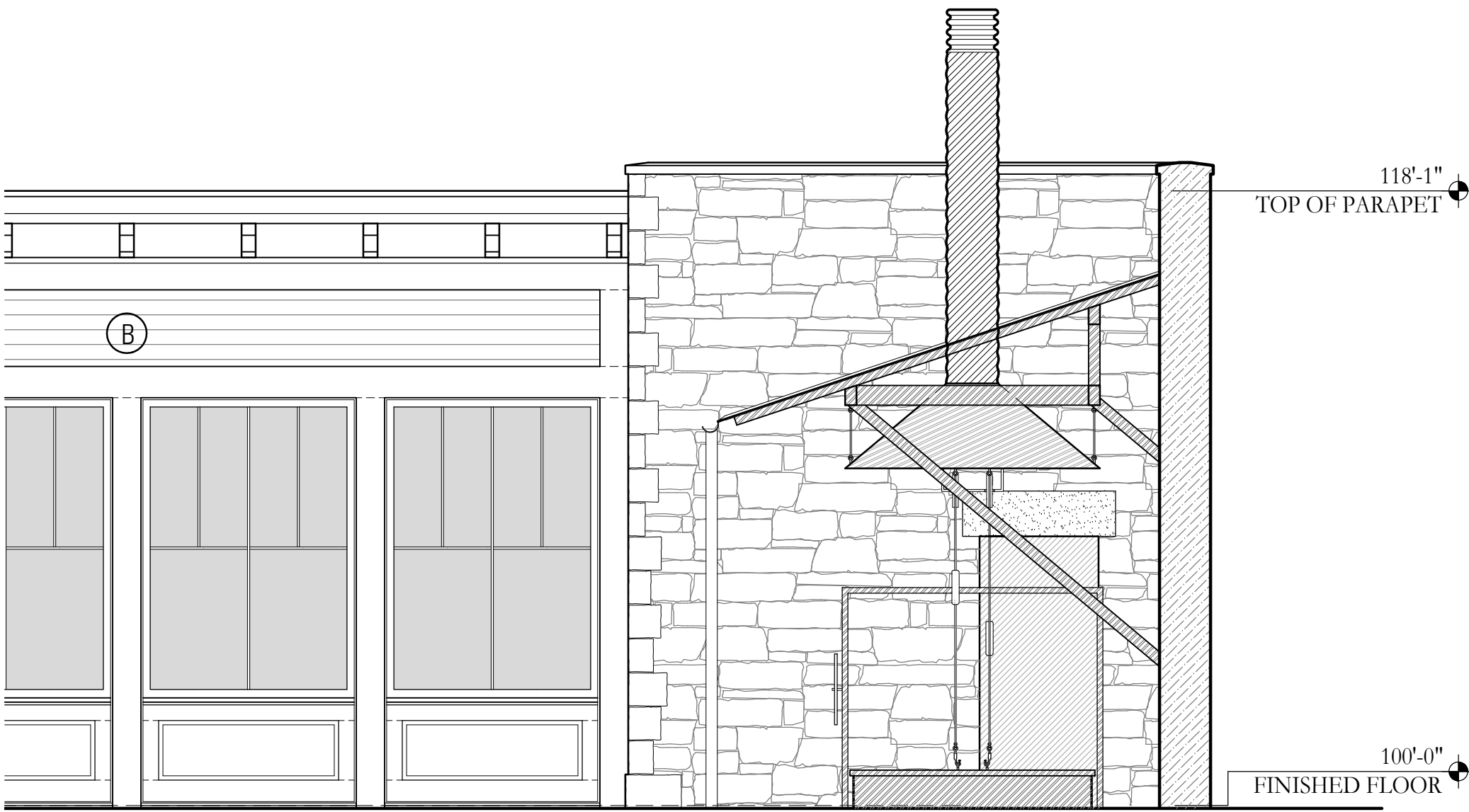
2 BBQ Pit West Elevation Scale: 1/4"=1'-0"
