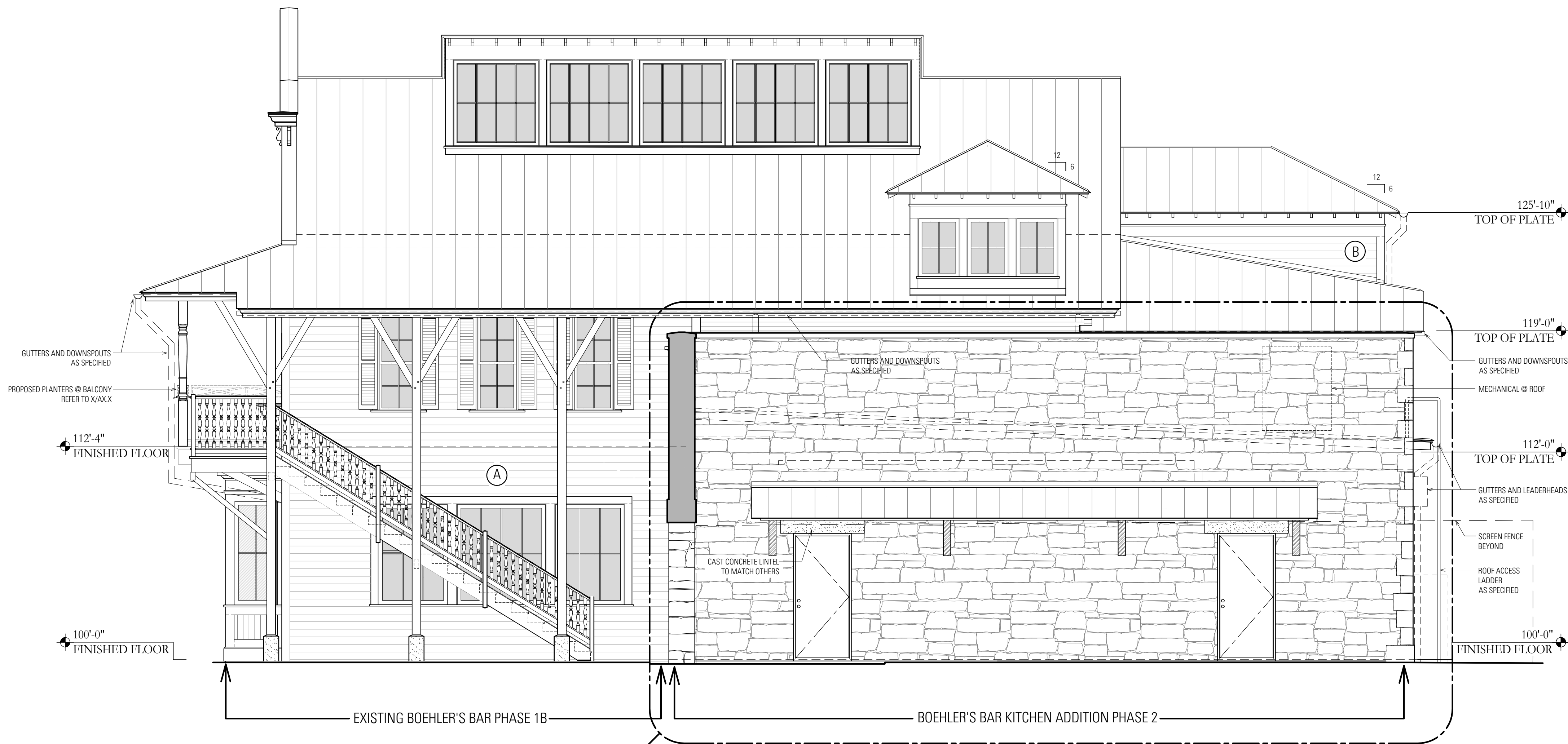
2 Boehler's Elevation - North Scale: 1/4"=1'-0"
