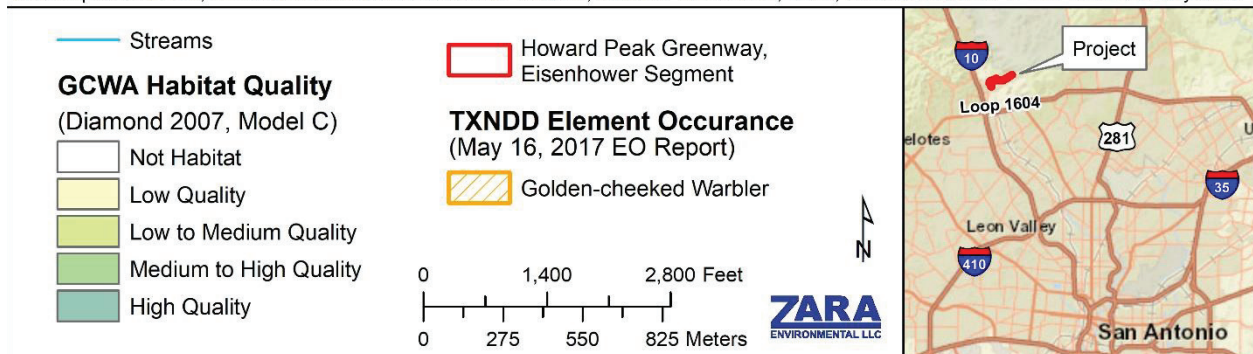
Figure 2. Diamond et al. 2010 Golden-cheeked Warbler habitat modeling data surrounding the project area.
