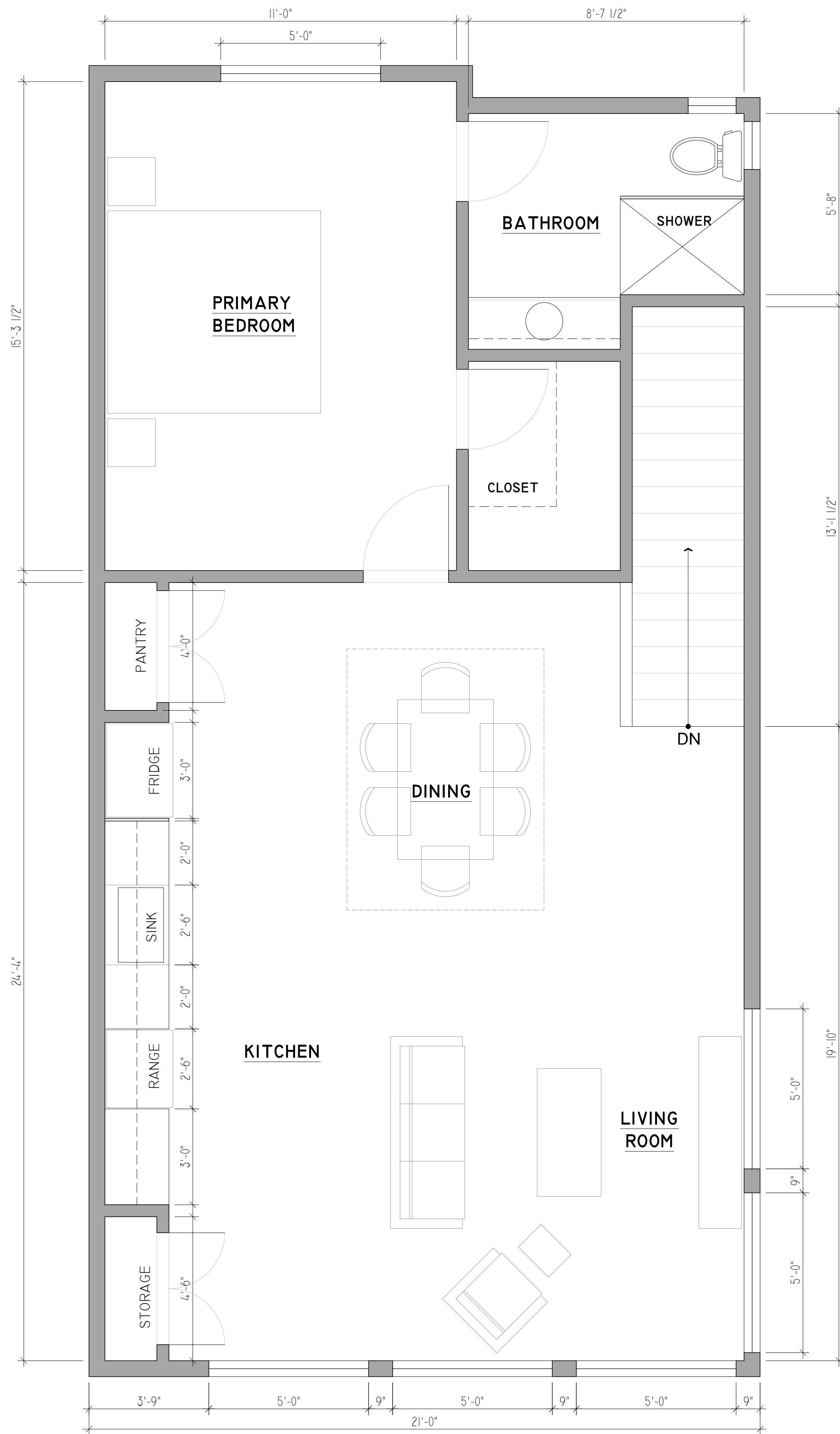
2ND FLOOR PLAN - OPT B SCALE: 3/8" = 1'-0"
