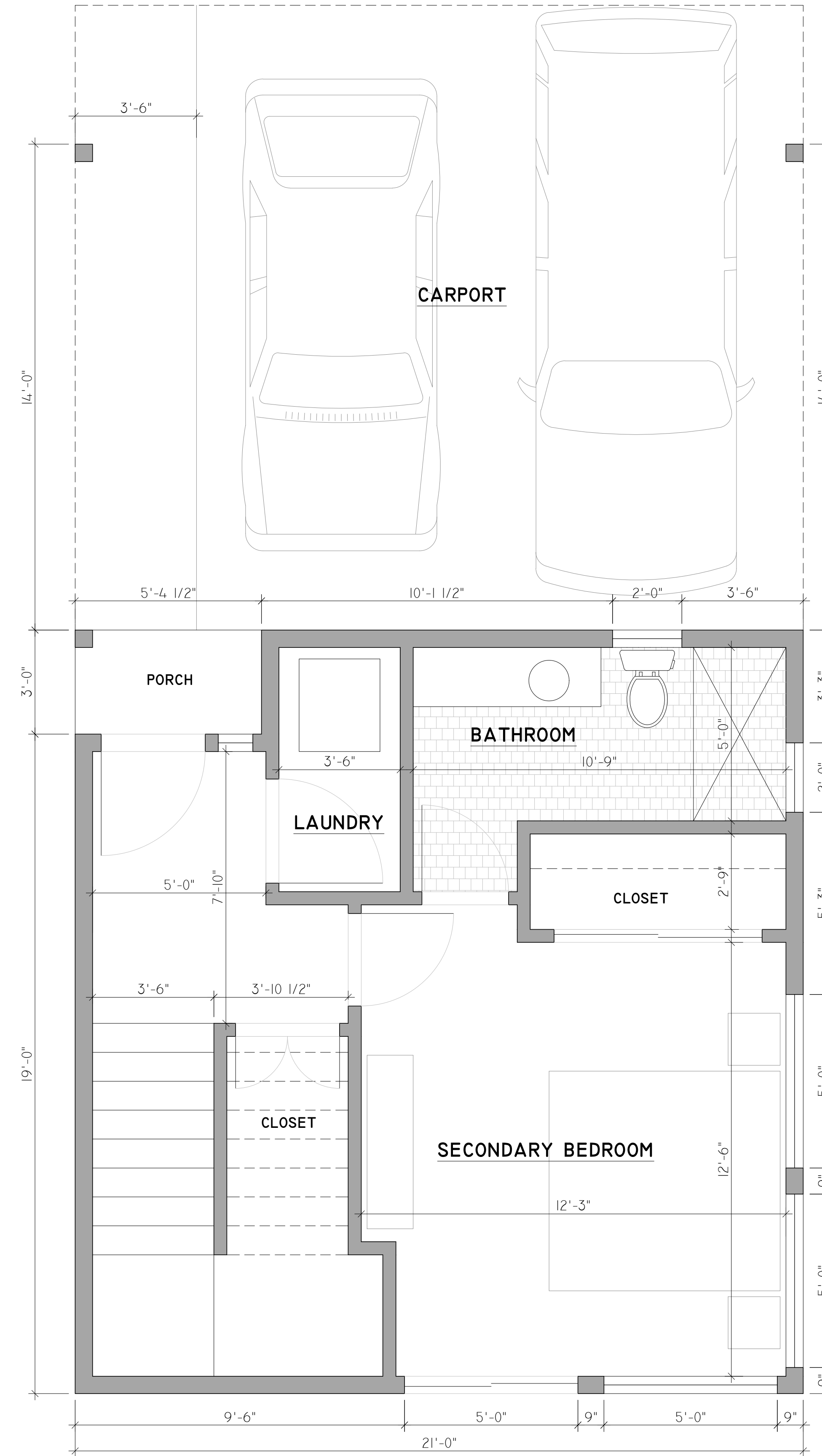
1ST FLOOR PLAN - OPT C SCALE: 3/8" = 1'-0"
