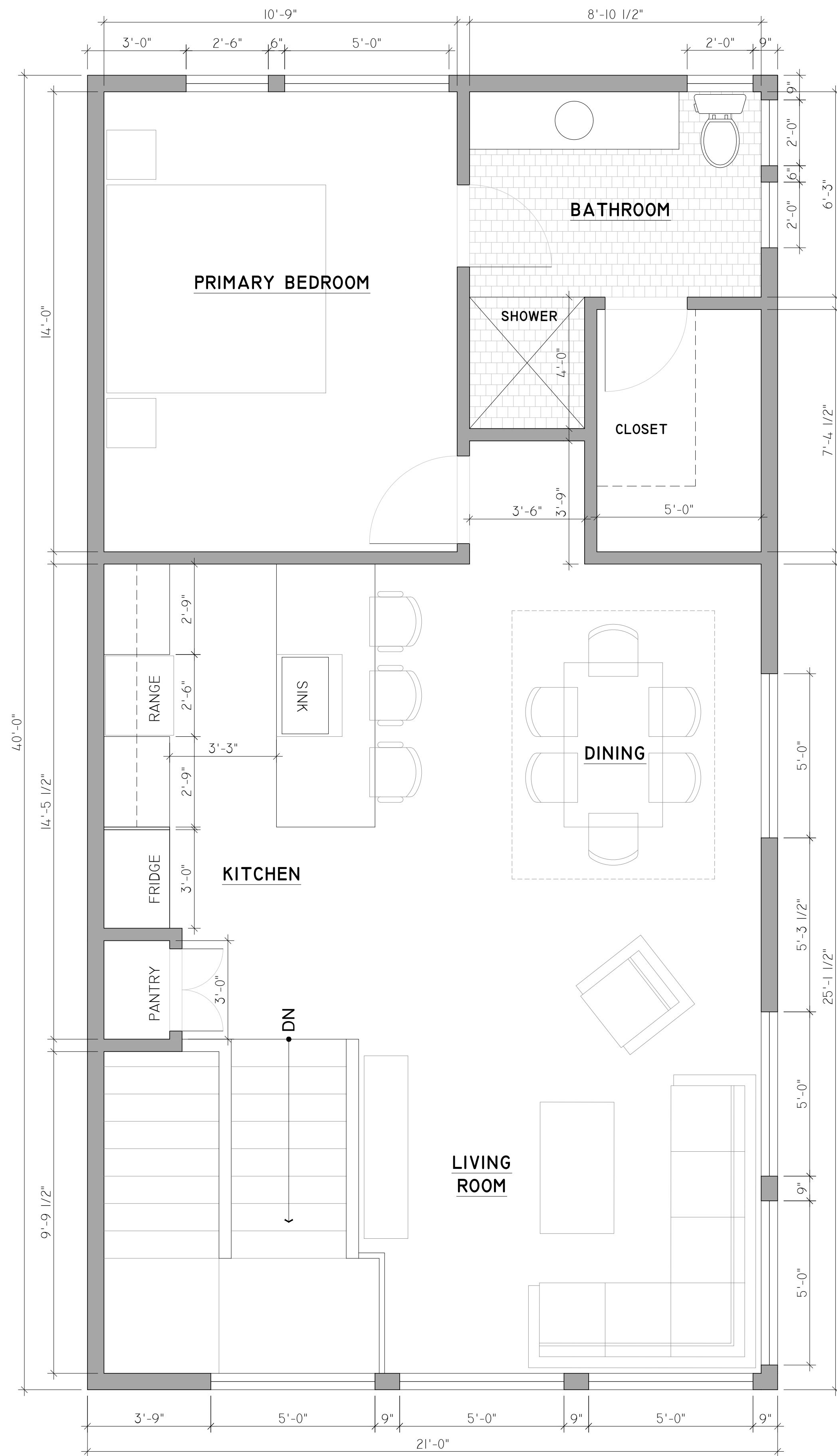
2ND FLOOR PLAN - OPT C SCALE: 3/8" = 1'-0"
