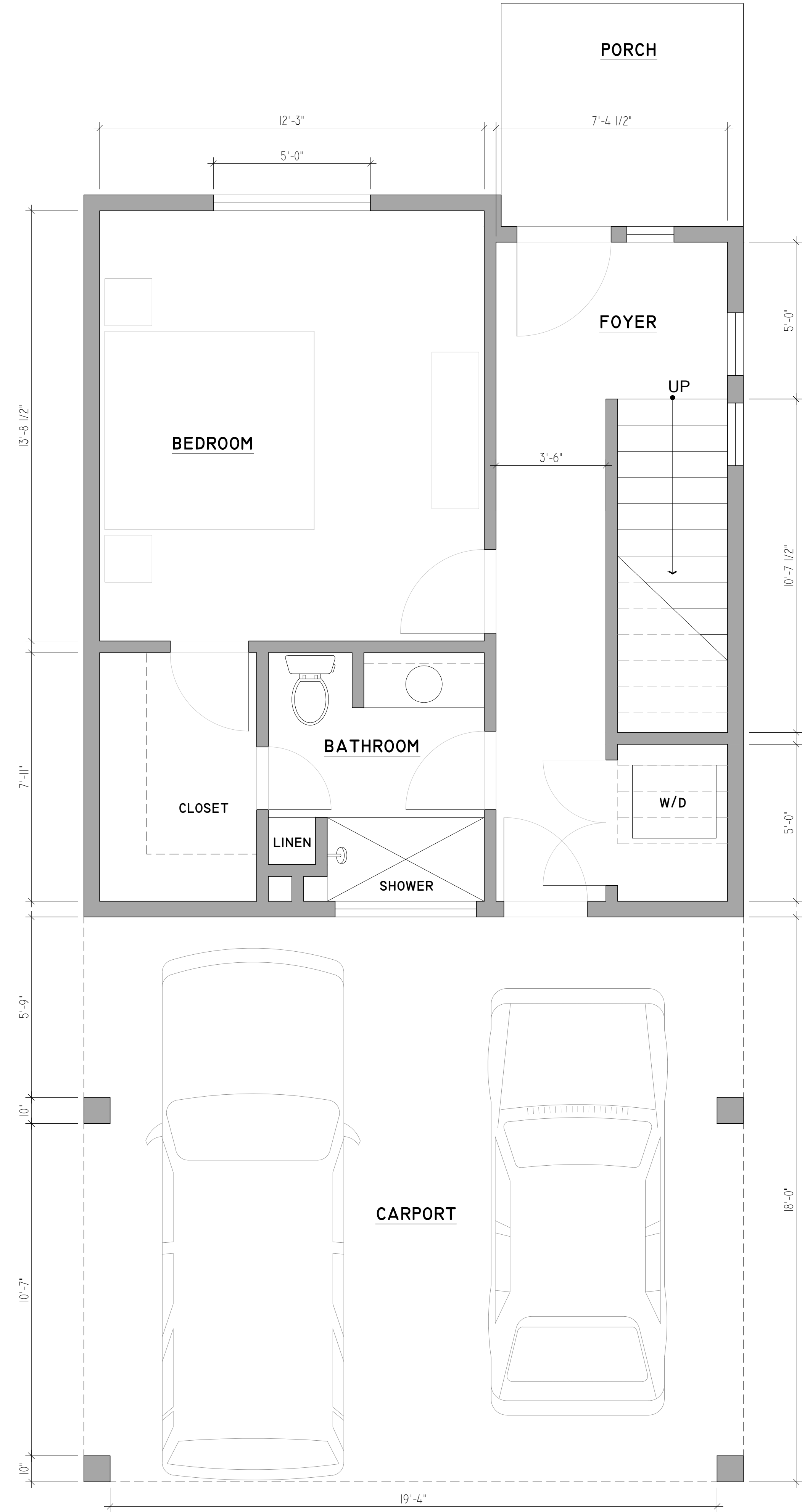
1ST FLOOR PLAN - OPT B SCALE: 3/8" = 1'-0"
